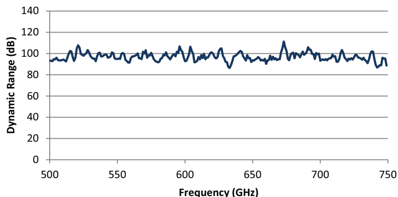
Typical Dynamic Range Plot of VDI WR1.5 Dual TxRx - 10 Hz IFBW
