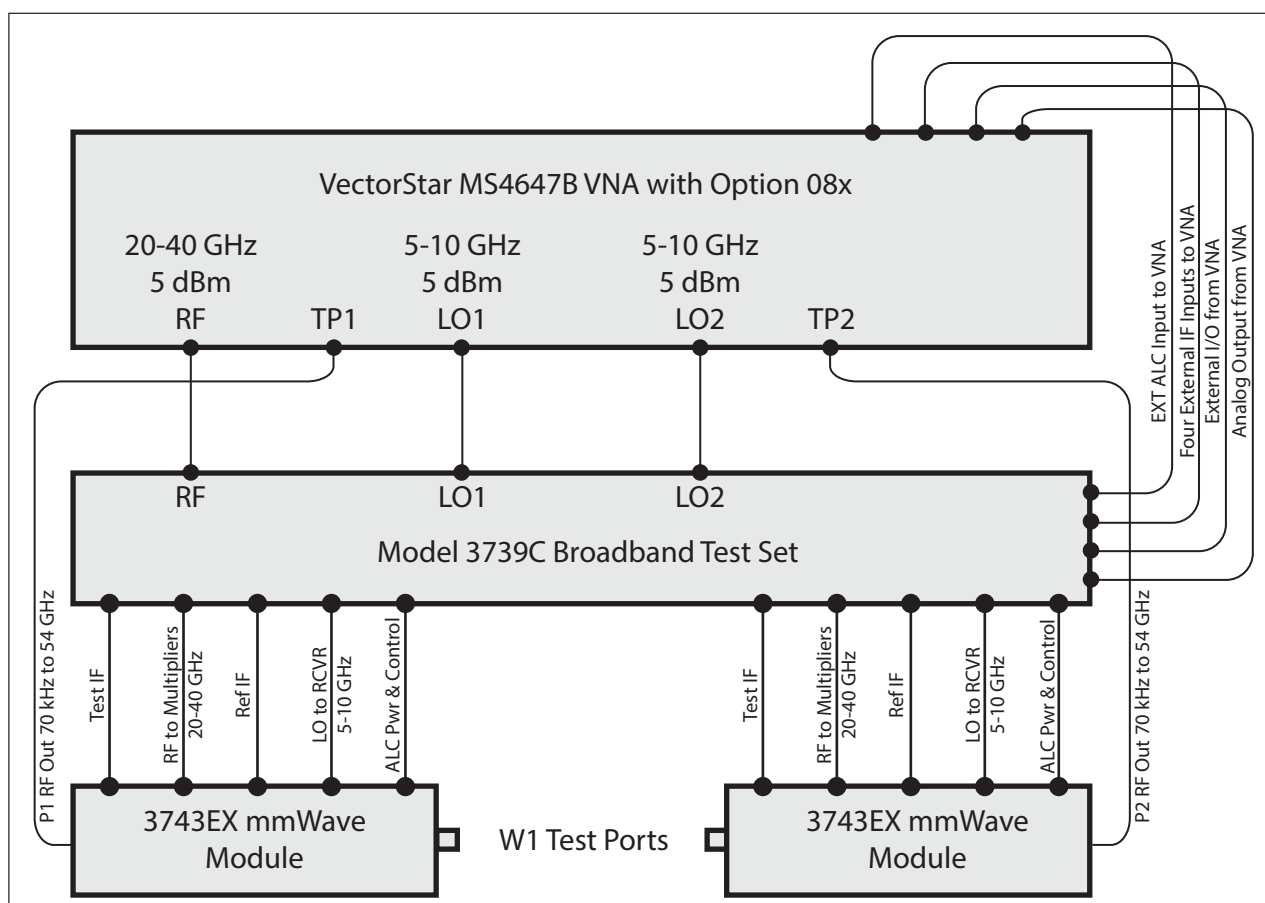
ME7838EX 2-port Broadband System
