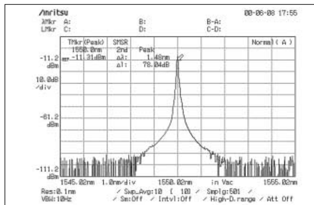
MG9541A optical output
