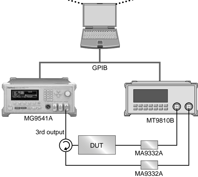
Coupler measurement example
