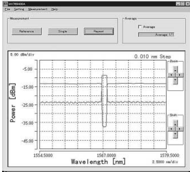
Coupler measurement example
