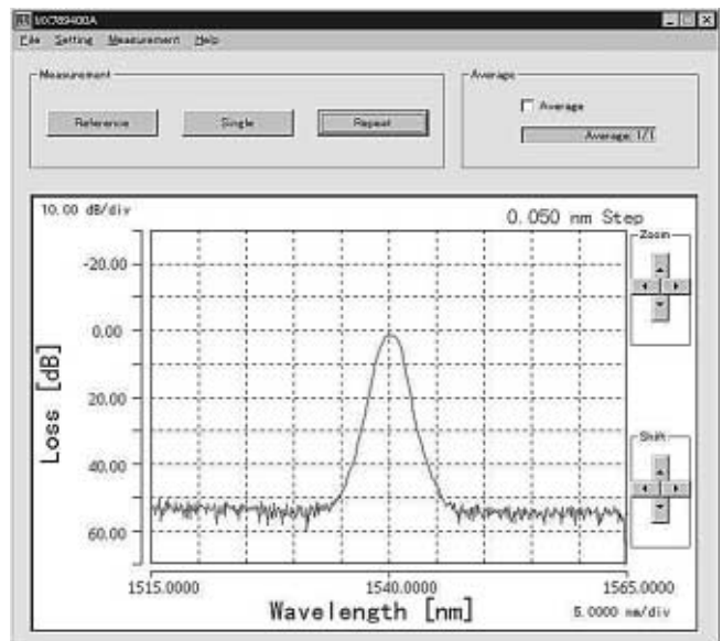
Optical filter measurement example
