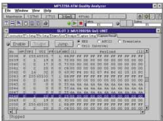
Cell capture display (hexadecimal)
