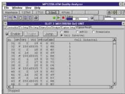
Cell capture display (cell interval)
