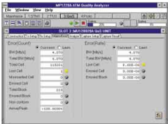
Measurement items for test cells
