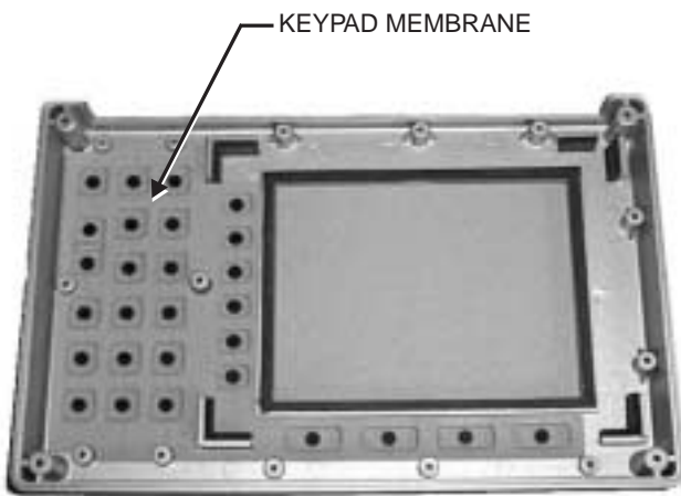
Figure 18. Front Panel Keypad Membrane
