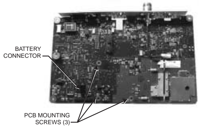
Figure 19. Main PCB
