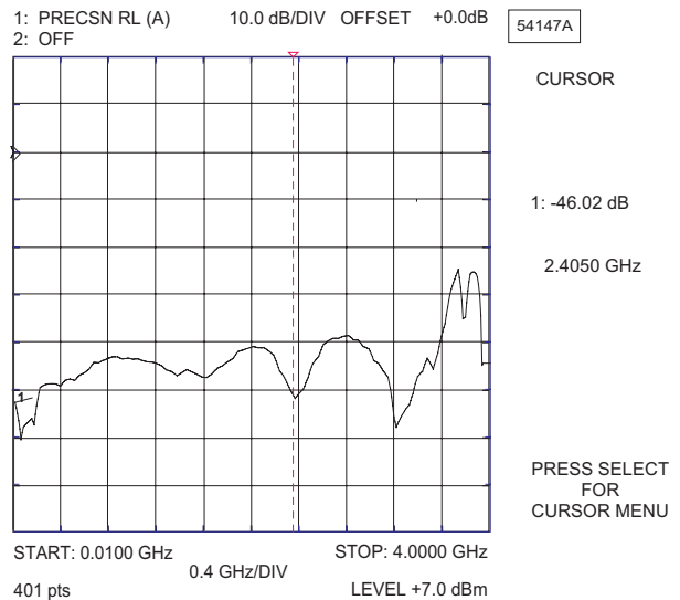
Figure 6. Direct Readout of the Precision Return Loss
