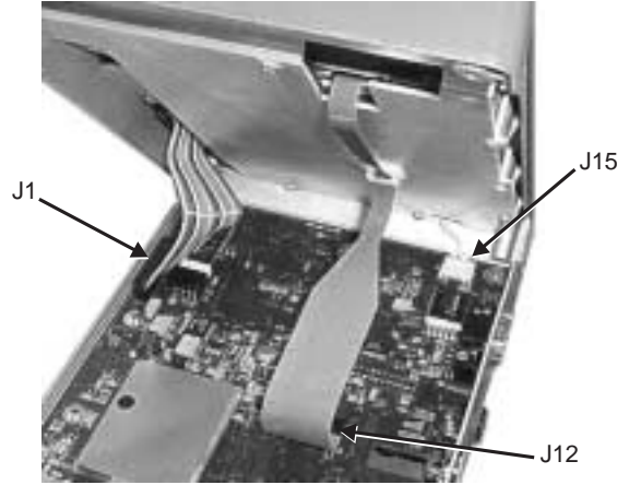
Figure 15. Site Master Front Panel Cable Connections
