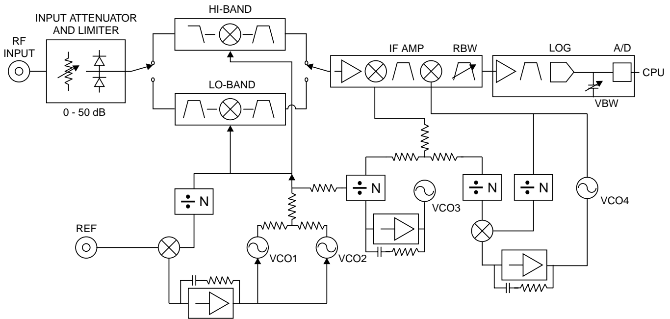
Figure 2. MS2711A Spectrum Analyzer Block Diagram
