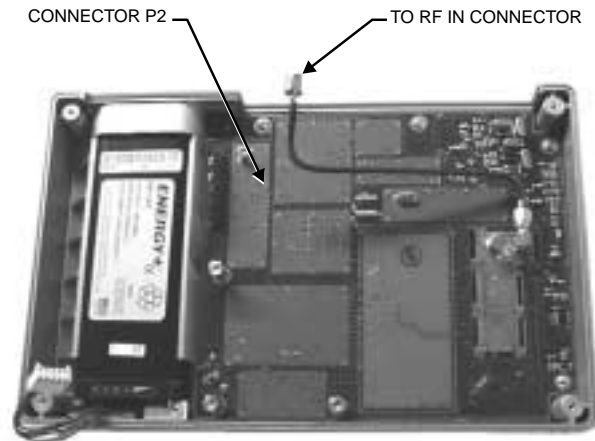
Figure 18. RF PCB
