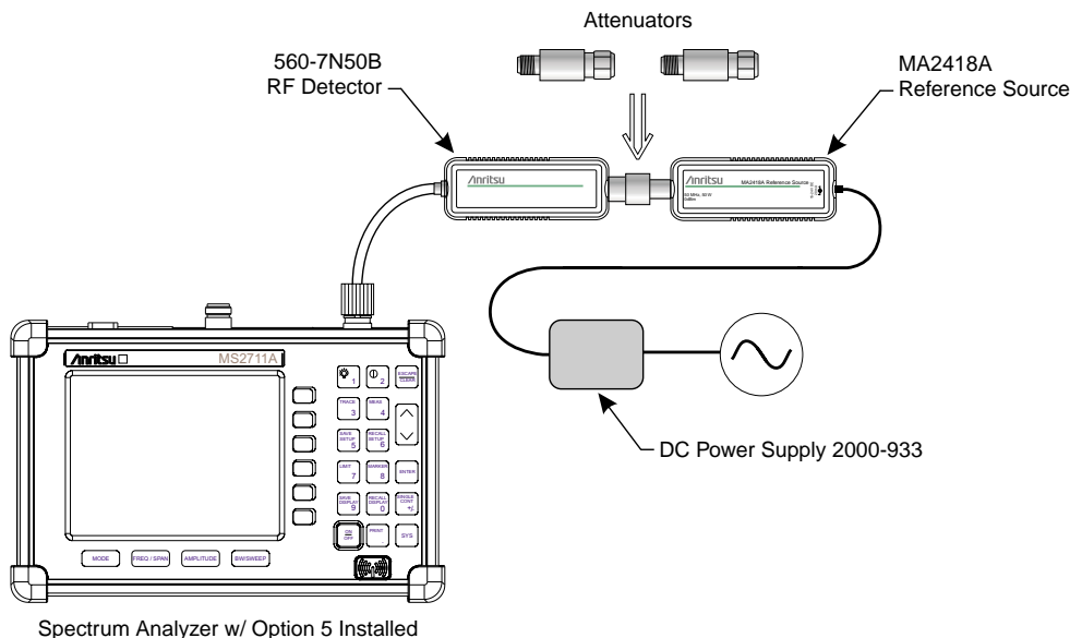
Figure 4. Power Monitor Verification
