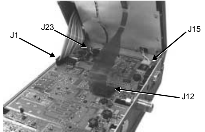
Figure 12. Spectrum Analyzer Front Panel Cable Connections
