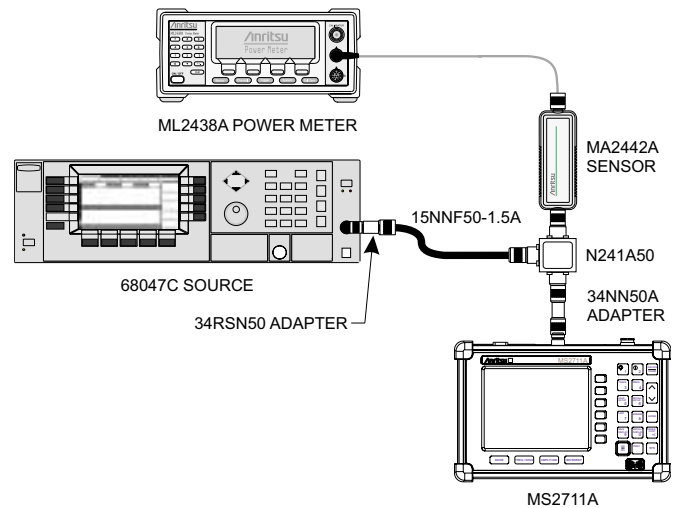
Figure 3. Measurement Accuracy Setup
