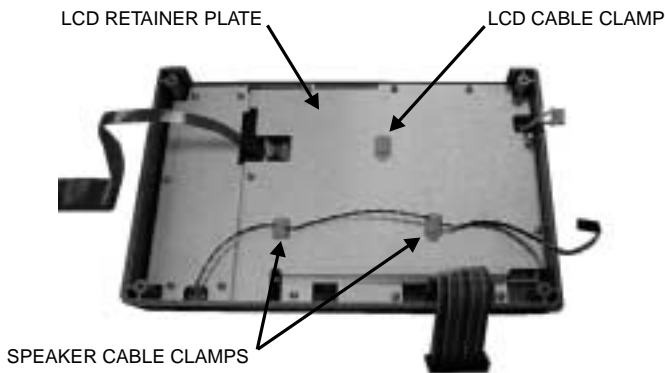
Figure 14. Front Panel Backing Plate
