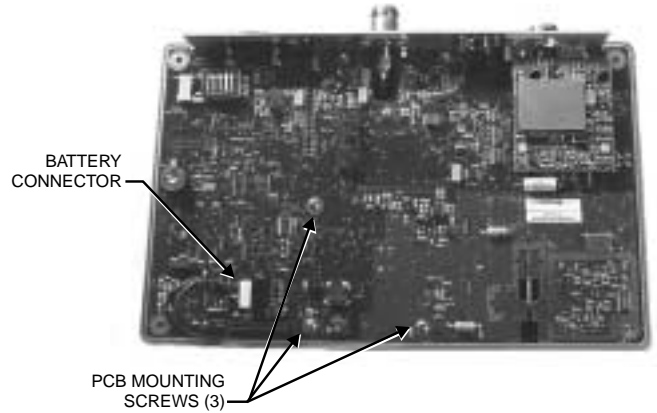
Figure 17. Control PCB
