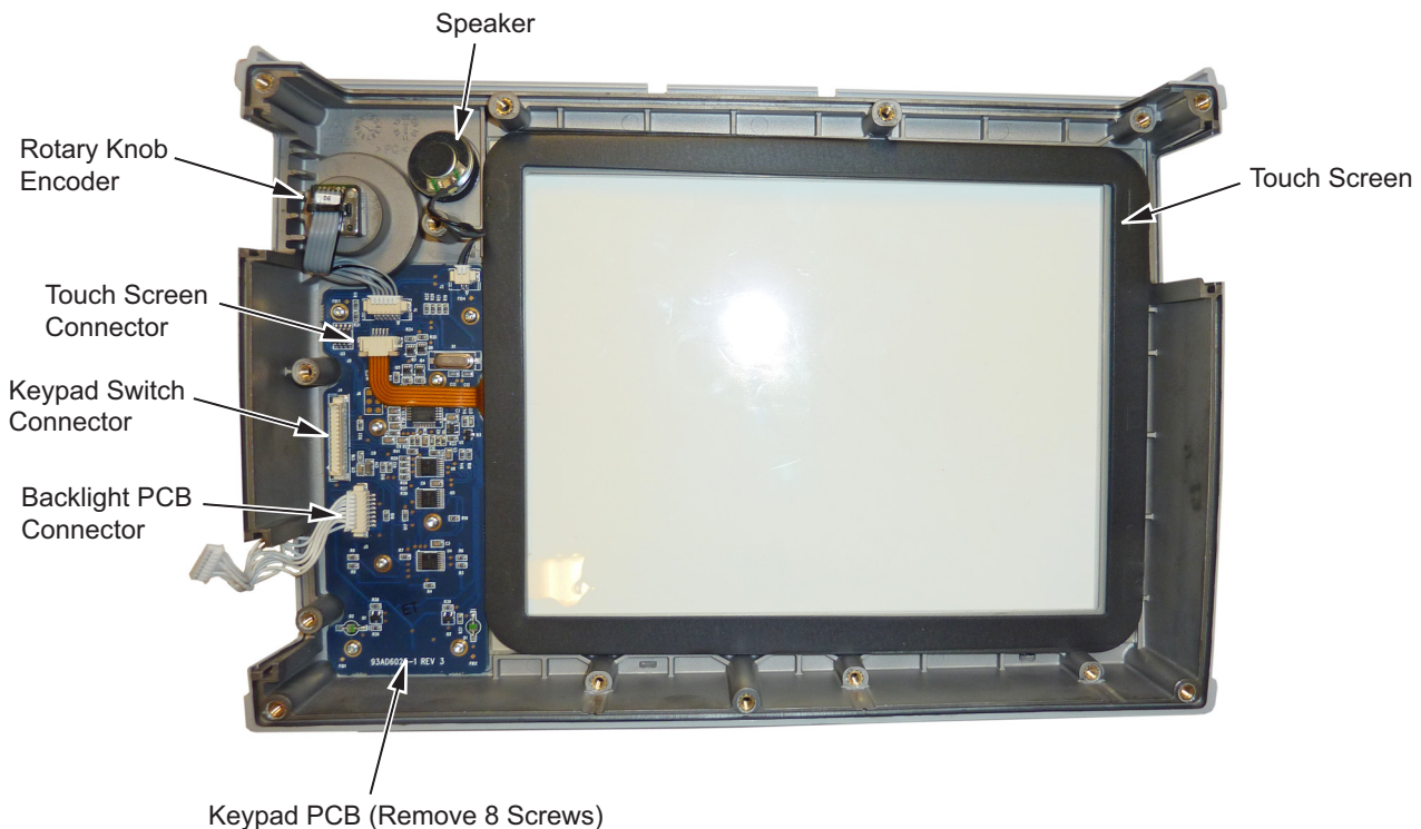
Figure 6-15. Front Panel Keypad Bezel
