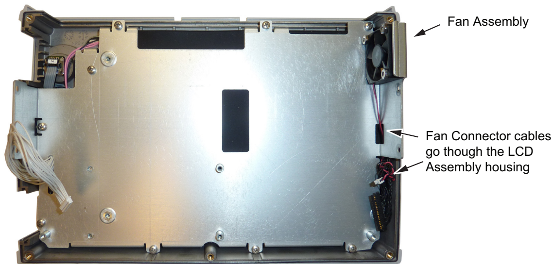
Figure 6-10. Front Panel Showing Fan Assembly
