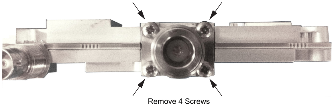
Figure 6-6. Remove 4 Screws
