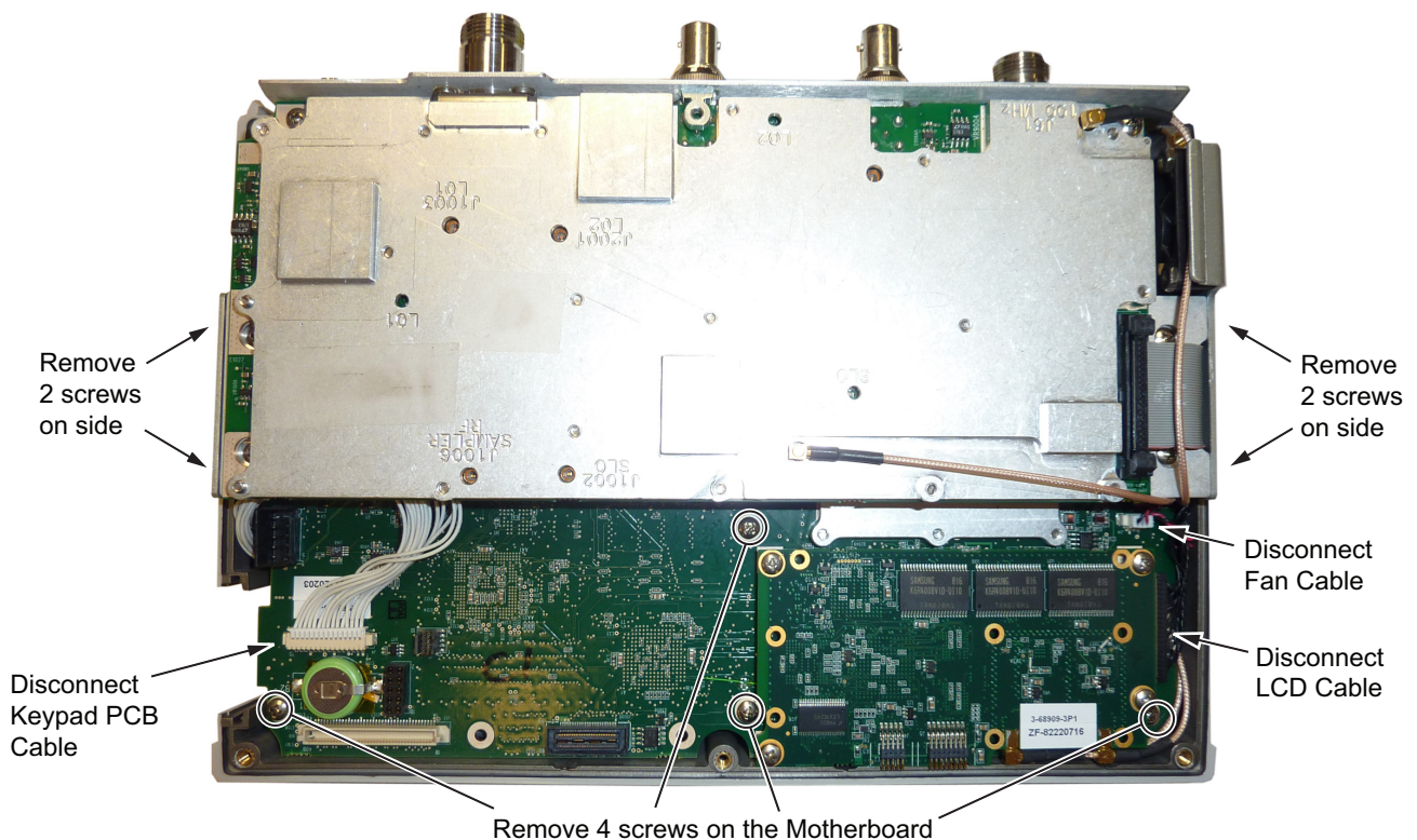
Figure 6-4. Removing the PCB Assembly out of the Case
