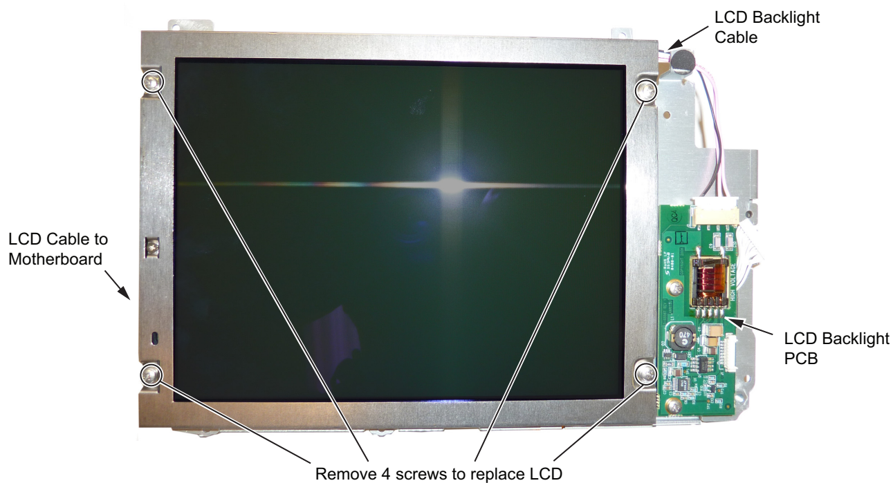
Figure 6-13. Replacing the LCD
