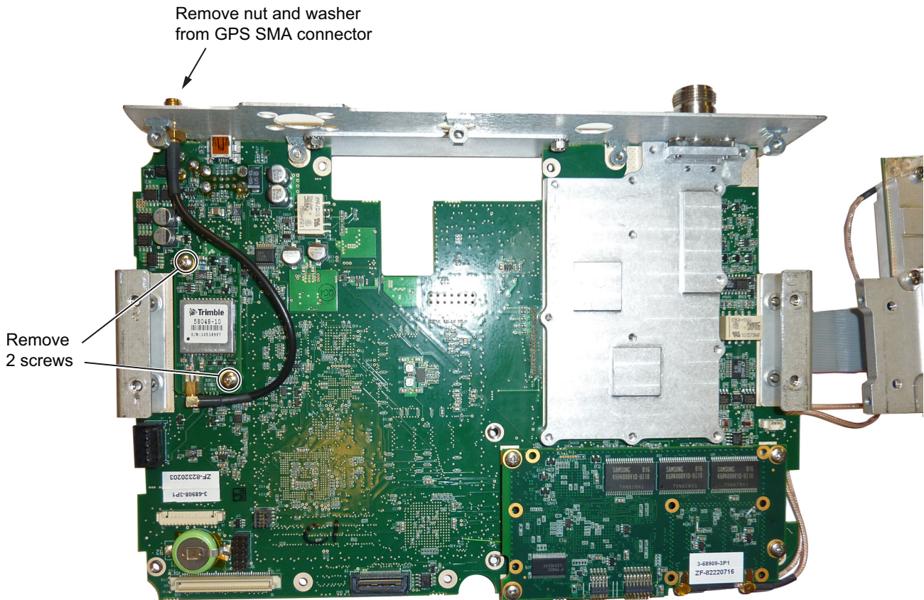
Figure 7-8. Removing the GPS PCB from the Motherboard (SPA PCB already removed)
