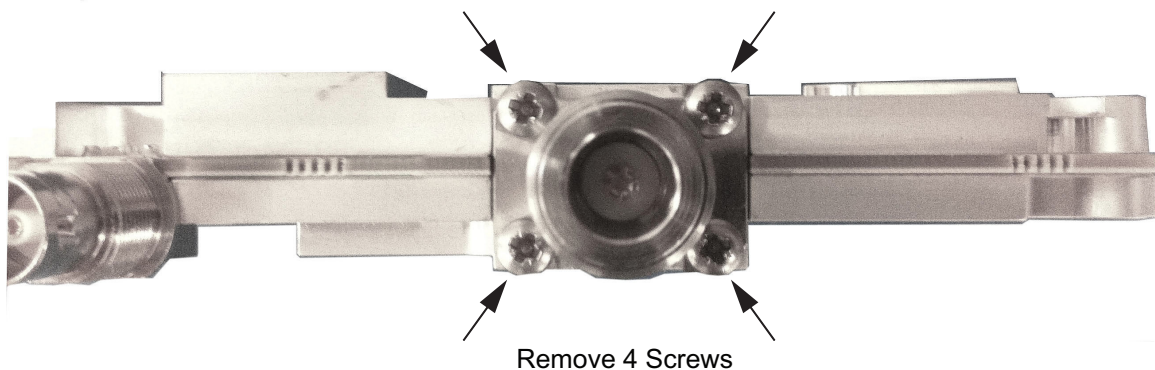
Figure 7-6. Remove 4 Screws
