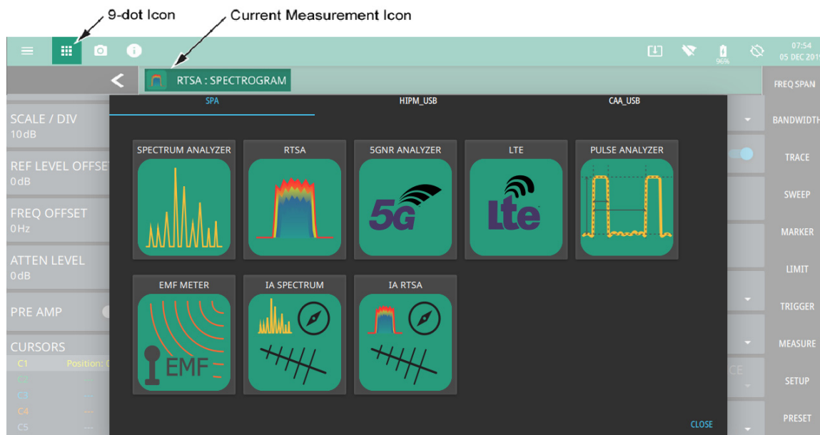
Figure 2-1. Example Analyzers
