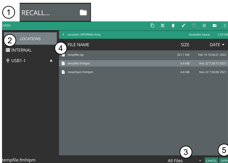
Figure 2-10. File Open Dialog
