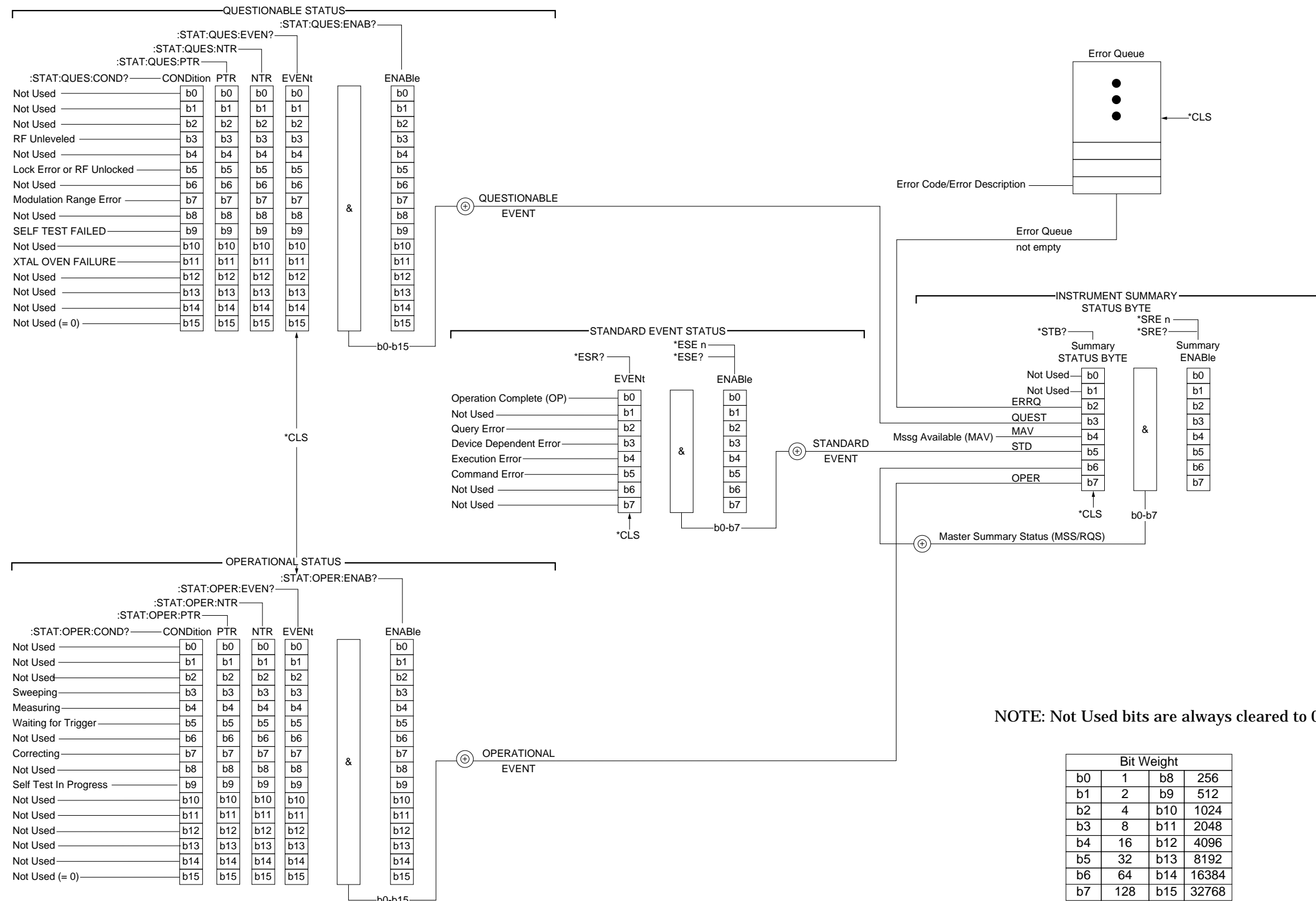
Figure 2-1. 680XXB Status-Reporting Structure
