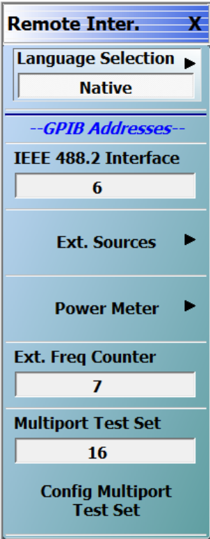
Figure 1-5. REMOTE INTERFACE (REMOTE INTER) Menu
