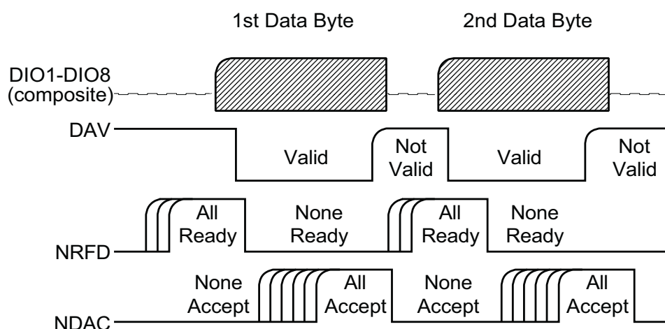
Figure 1-2. Typical GPIB Handshake Operation
