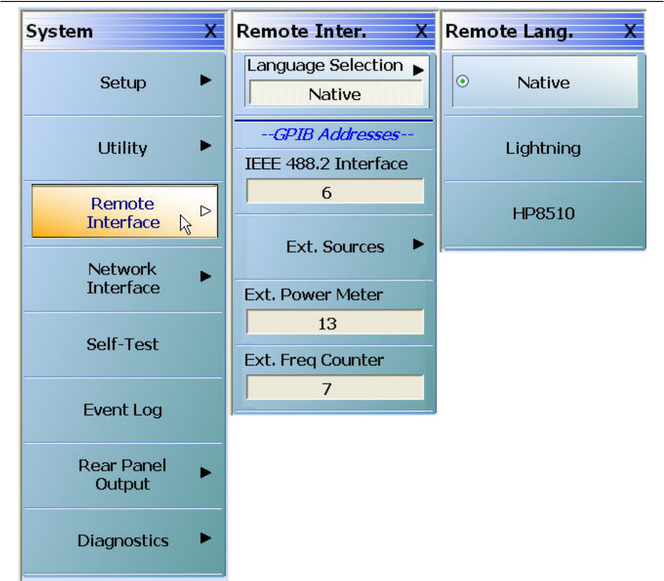
Figure B-5. VectorStar REMOTE LANGUAGE Setup Menus
