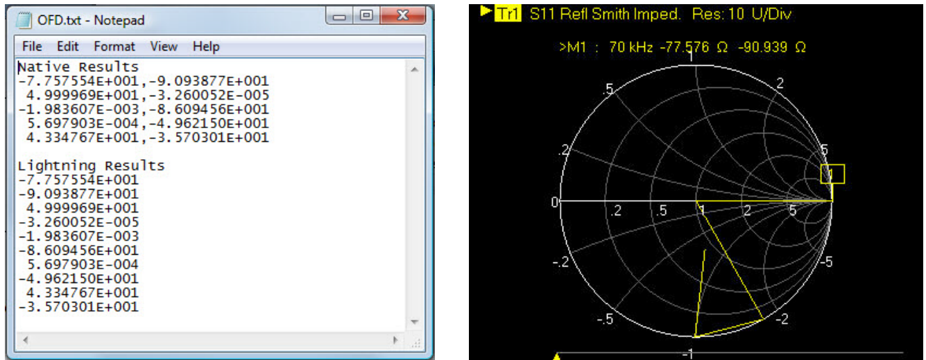
Figure C-19. Example 4 – Listing and Graph Outputs
