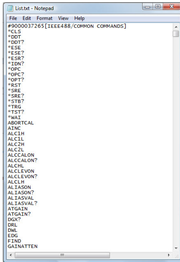
Figure D-27. List of all commands supported by the MS464xB Series VNA
