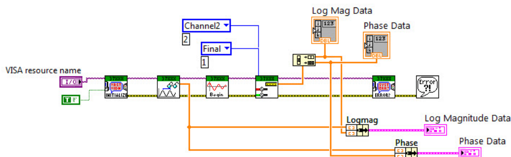
Figure D-54. VI Block Diagram
