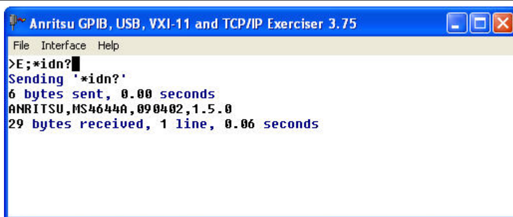
Figure A-8. *IDN? Query and Output Results
