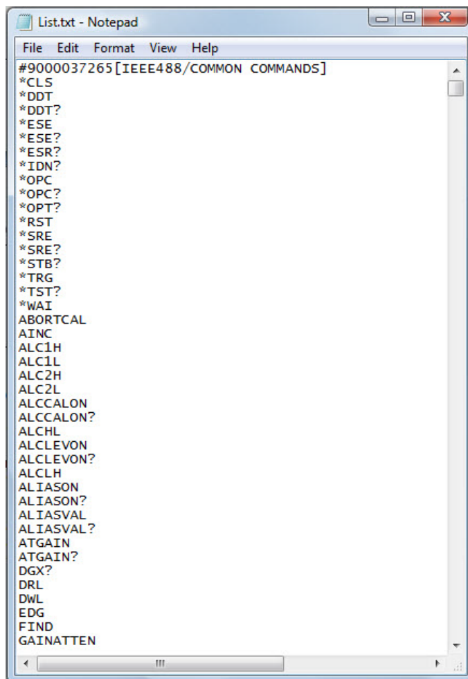
Figure C-17. Example 3 – VectorStar Command Listing
