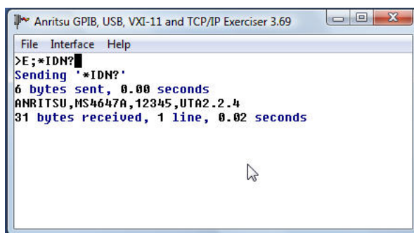
Figure D-16. Anritsu GPIB, USB, VXI-11, and TCP/IP Exerciser
