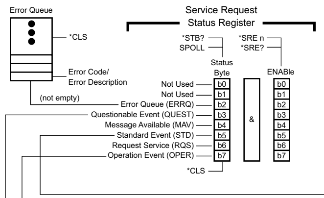
Figure B-27. Example 3 – Service Request Status Register – VectorStar Status Register (1 of 2)
