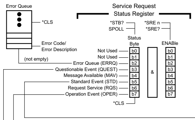
Figure D-25. The Service Request Status Register
