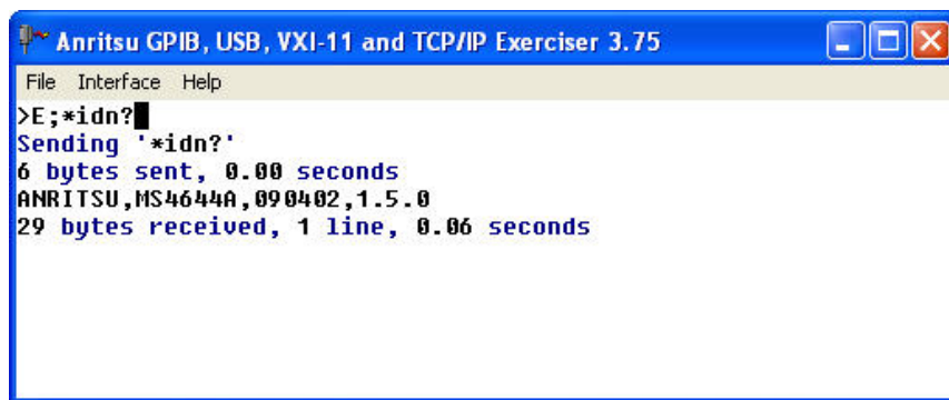
Figure B-8. Using WGPIB with *IDN? Command
