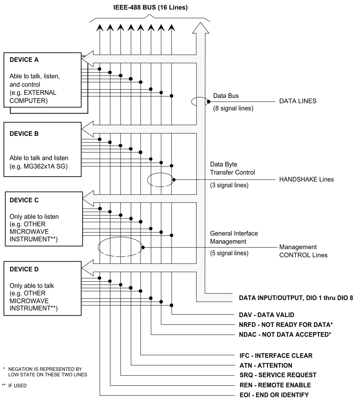
Figure 1-1. GPIB Interface Connection and Bus Structure
