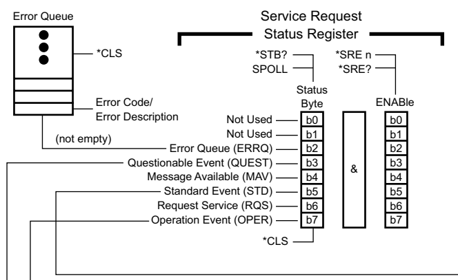
Figure D-81. MS464xB Service Request Status Register
