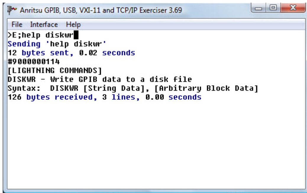
Figure B-30. WGPIB Help
