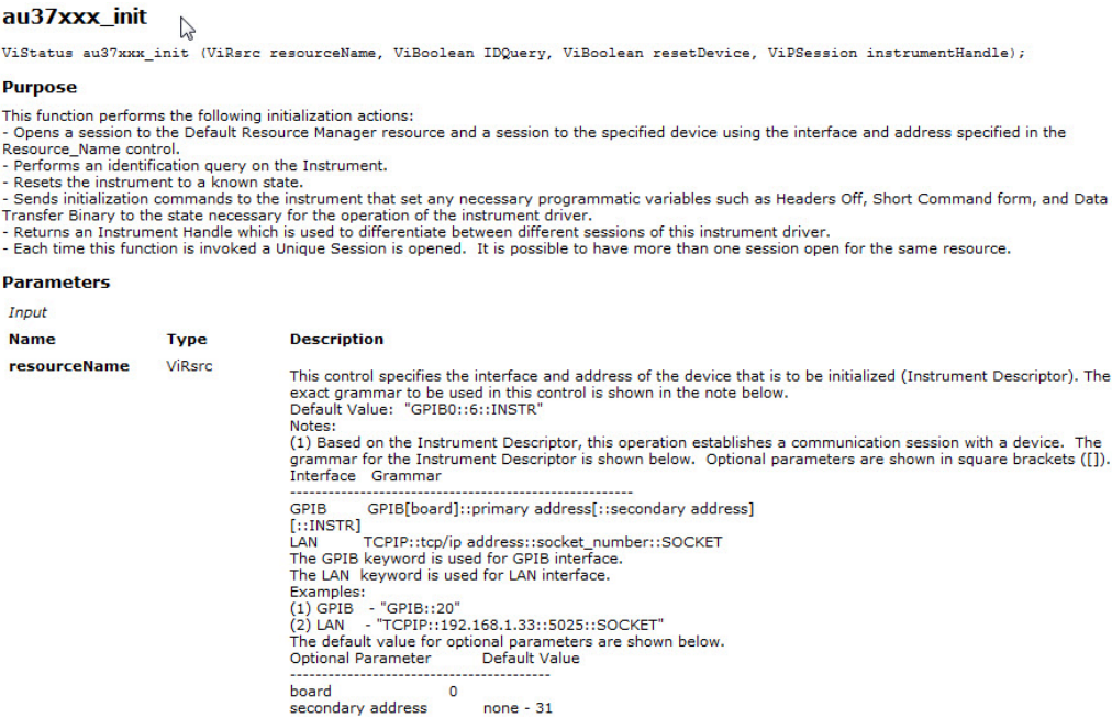
Figure D-12. au37xxx LabWindows/CVI Driver Function Help File
