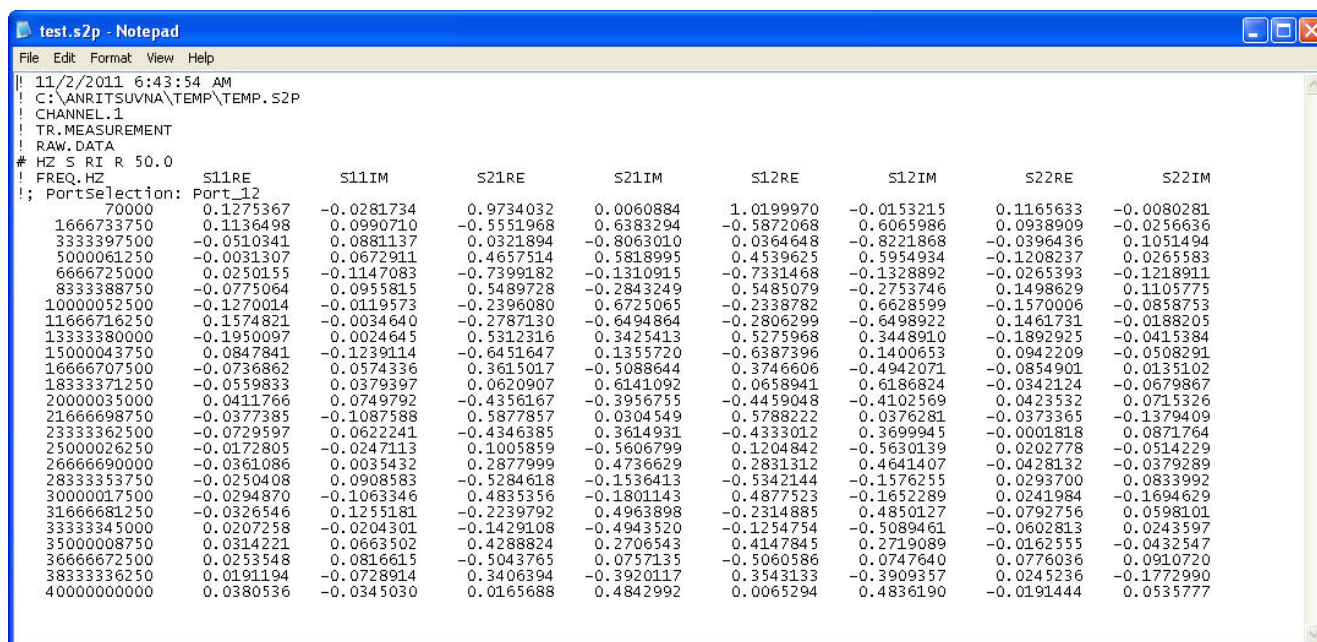
Figure A-35. Example 7 – S2P File Transferred to the PC Controller
