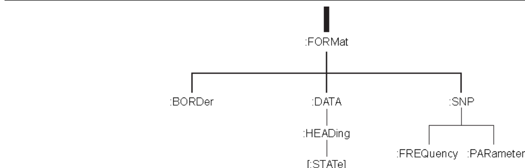
Figure 2-2. SCPI :FORMat Subsystem
