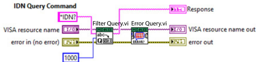
Figure D-23. Example 2 – Block Diagram – Send *IDN? Command
