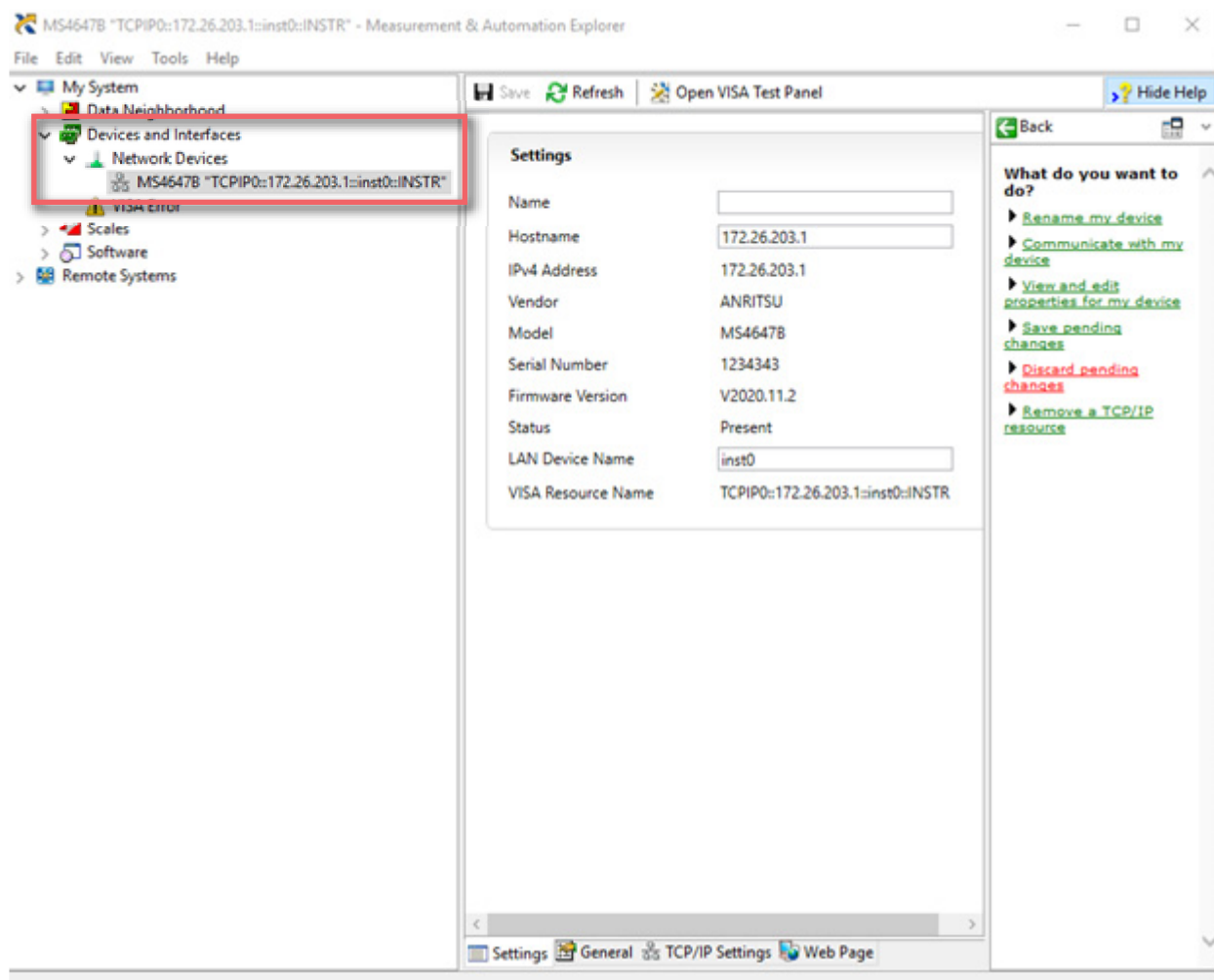
Figure D-18. Measurement & Automation Explorer Window – MS 46524B Connected to LabVIEW
