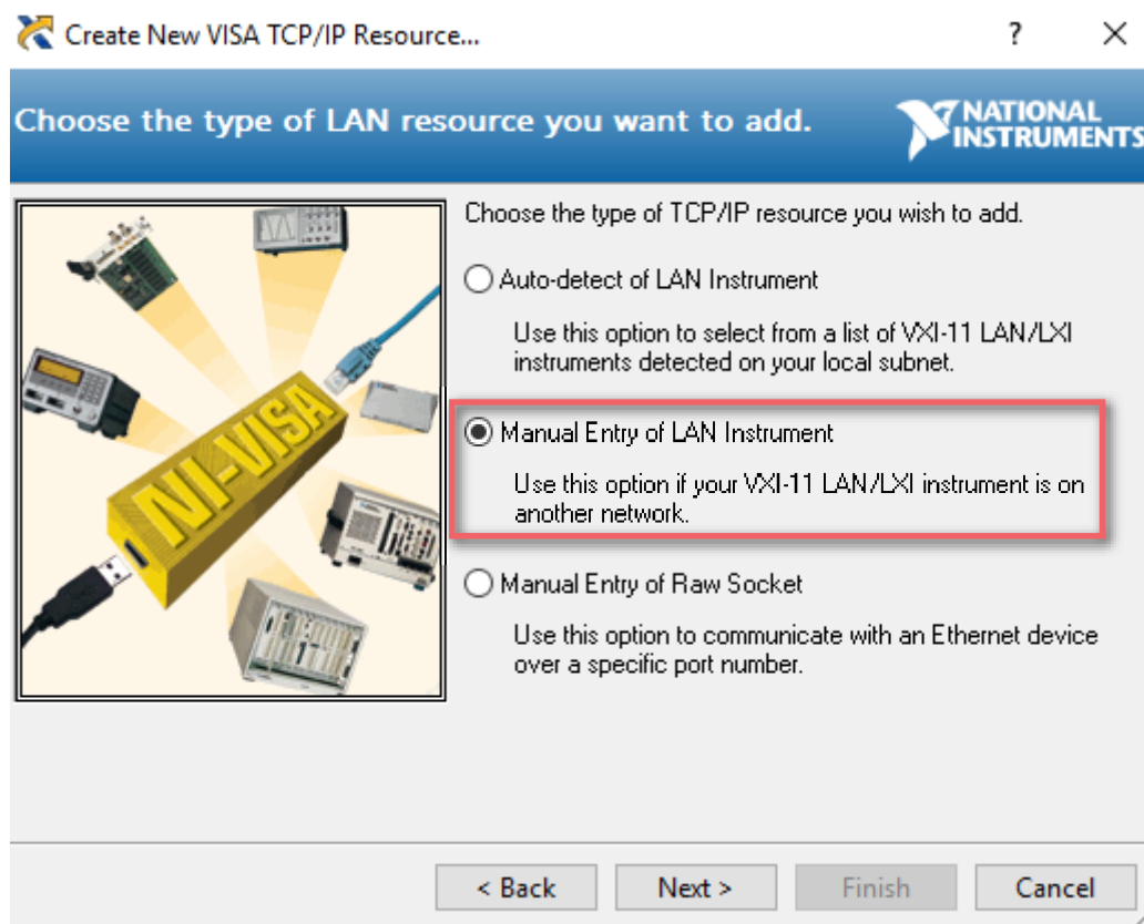
Figure D-13. Manually Create New VISA TCP/IP Resource
