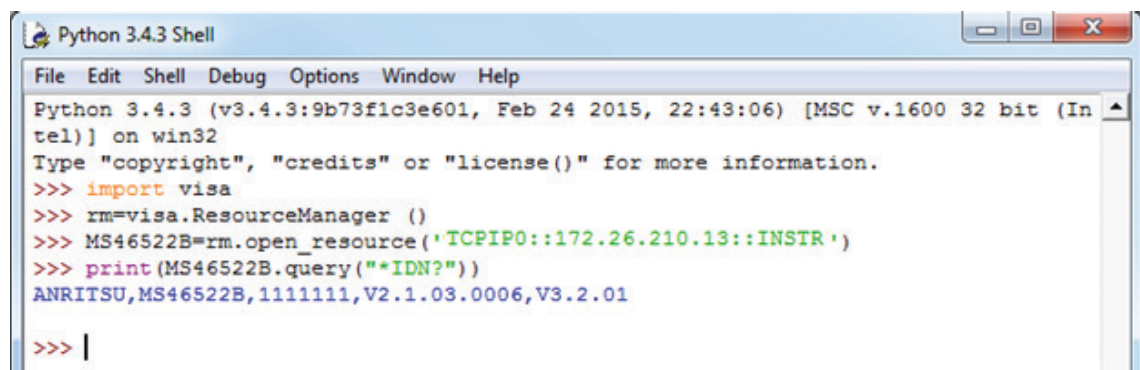
Figure 1-18. Instrument Identification Inquiry
