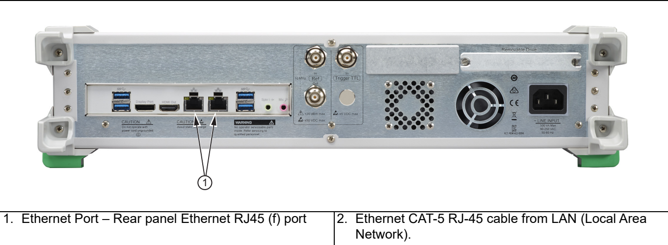
Figure 1-5. MS46322A/B Network Connection
