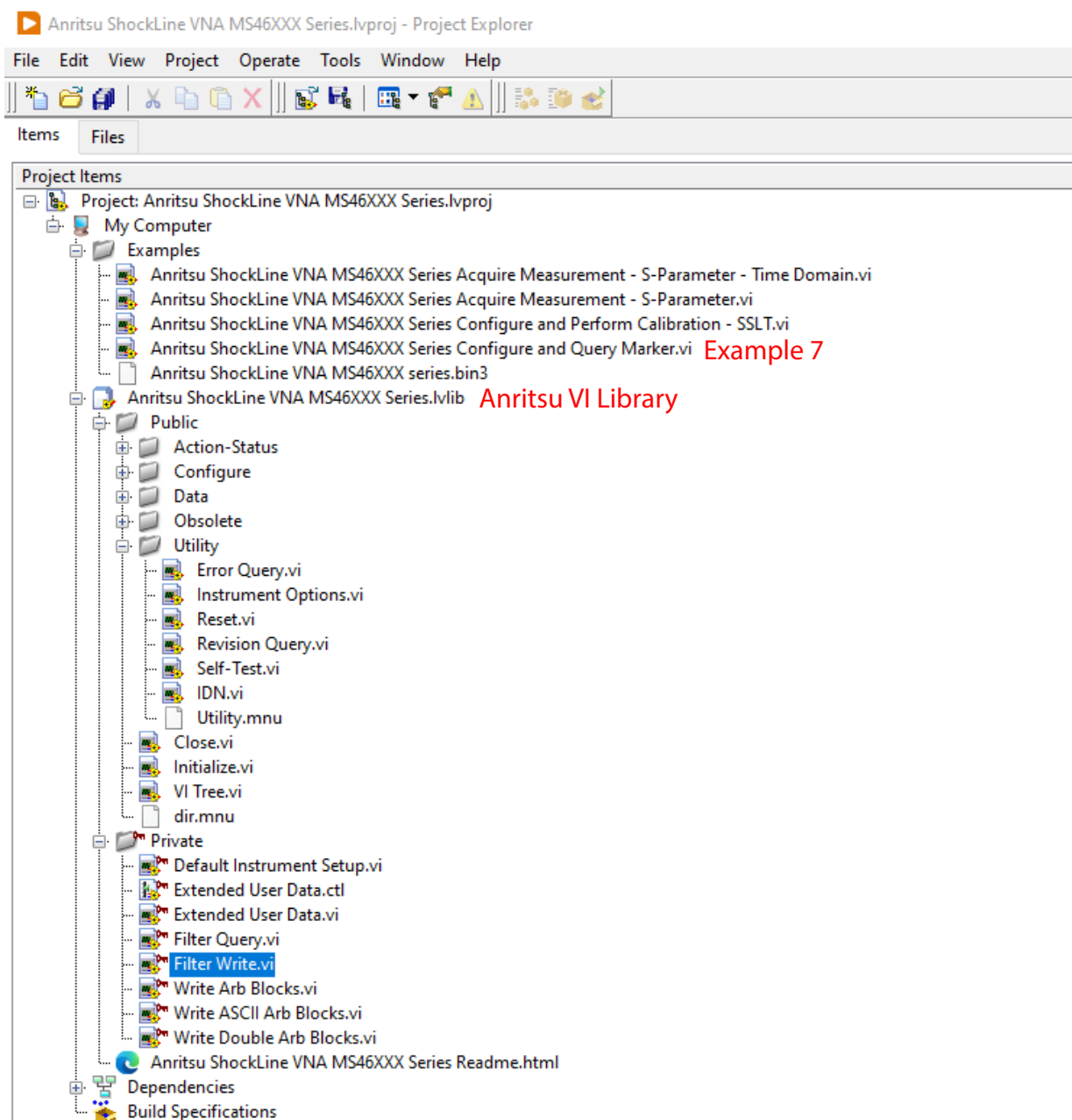
Figure D-19. Anritsu Examples and VI Directory
