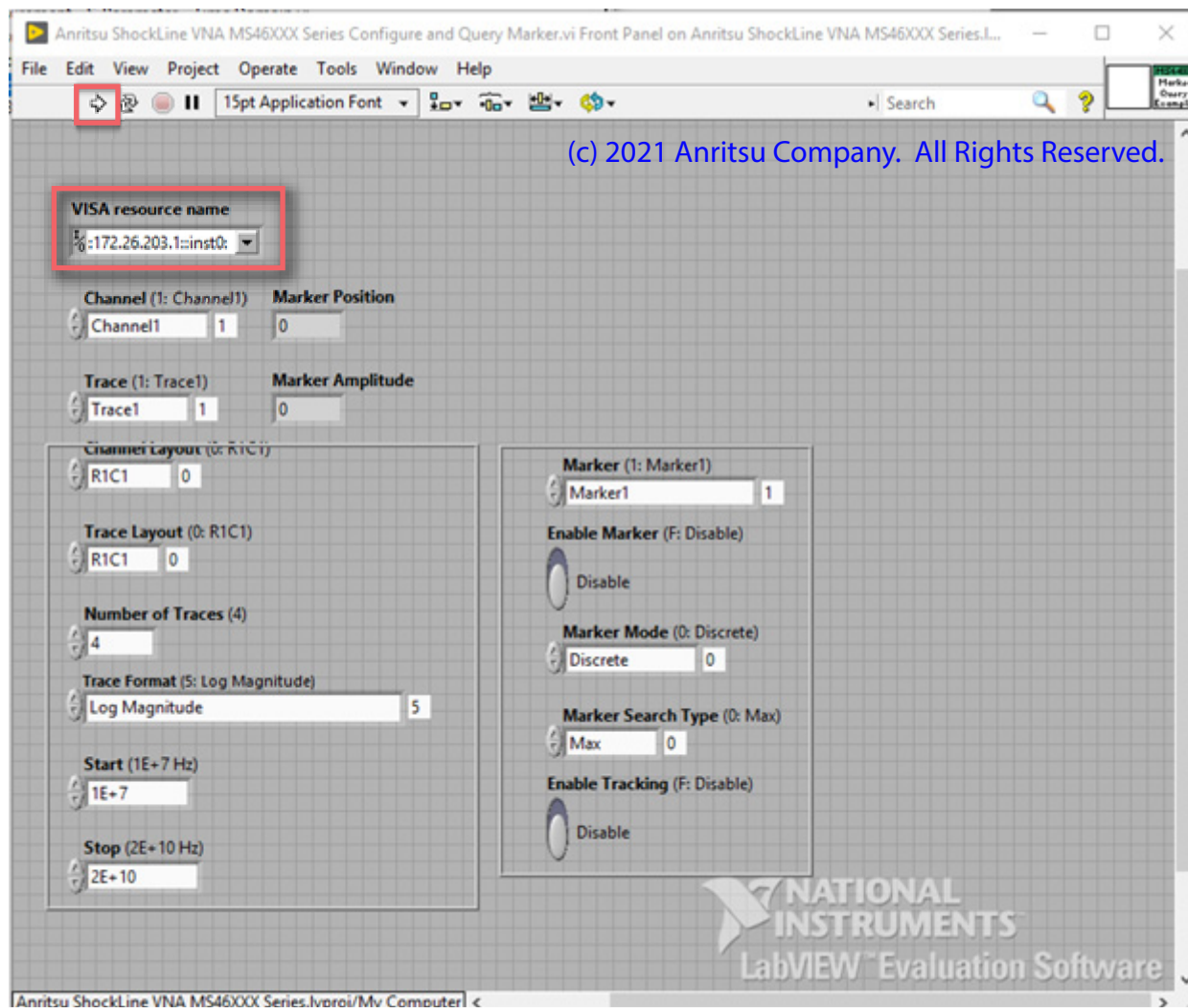
Figure D-37. Example 7 – LabView Front Panel – Connect to VISA Resource
