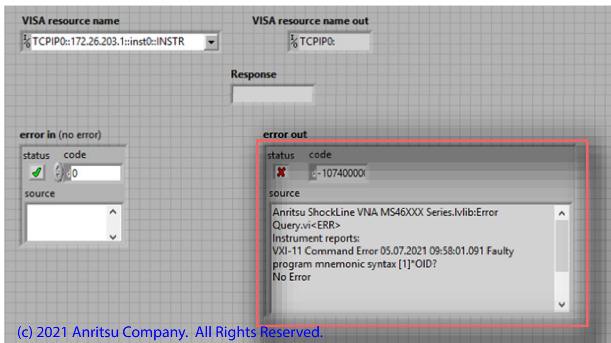
Figure D-26. Example 3 – LabView Front Panel – Error Message Displayed
