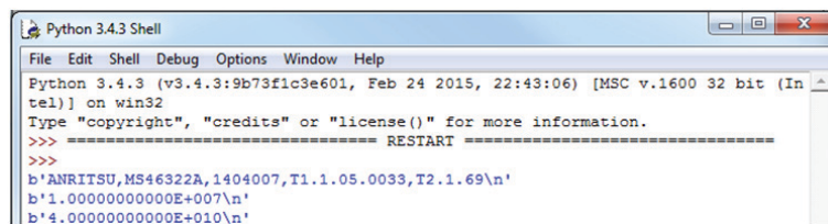
Figure 1-11. Python Script with SCPI Commands for the MS46122A/B
