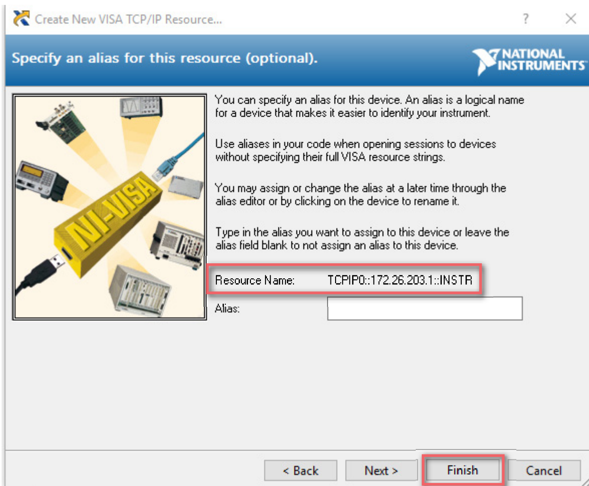
Figure D-17. Display the VISA VXI-11 Resource Name
