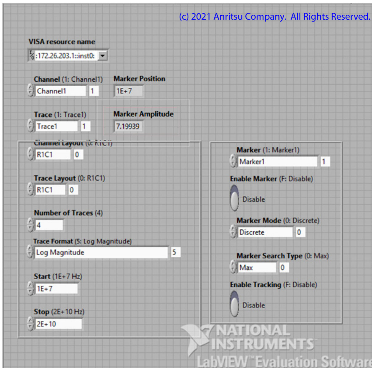
Figure D-39. Example 7 – LabView Front Panel – Result After Run
