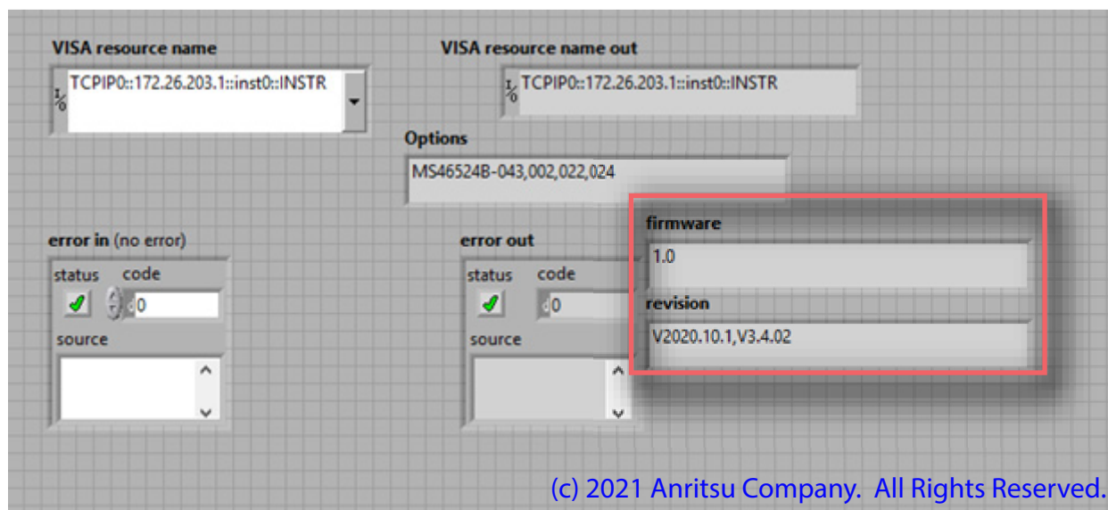
Figure D-22. Example 1 – LabView Front Panel – VNA Firmware and Revision Information Displayed
