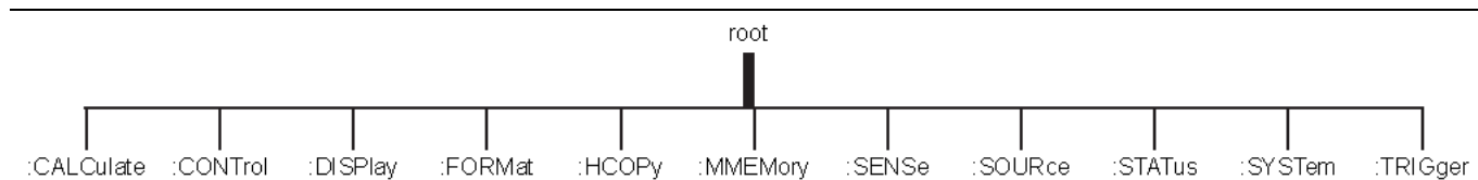
Figure 2-1. Shockline™ VNA Top-Level SCPI Command Tree
