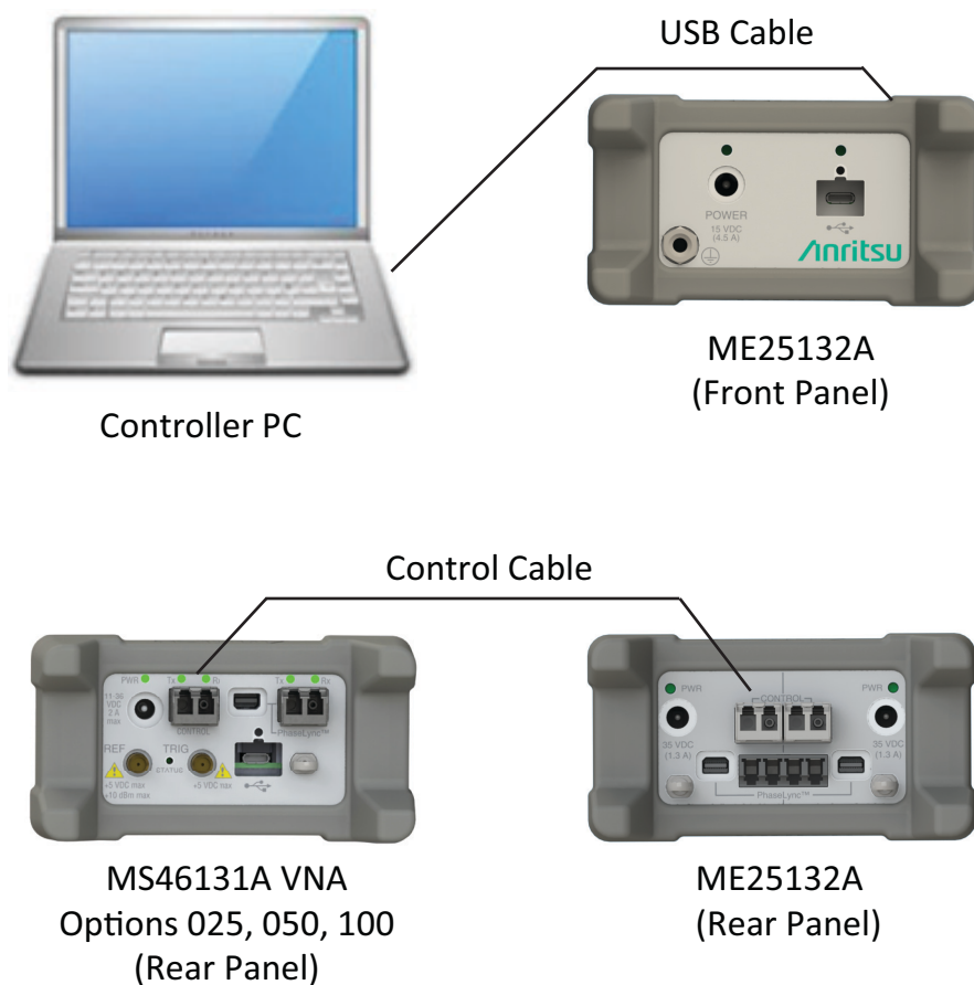
Figure 1-15. Connecting the ShockLine VNA (ME7869A) to Required External Control PC
