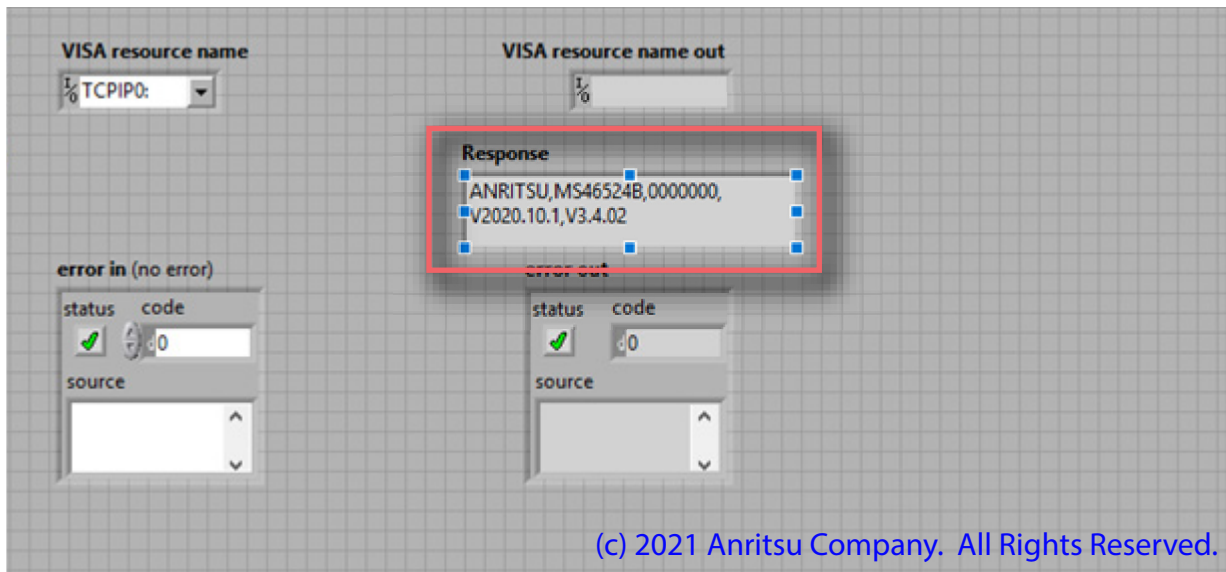
Figure D-24. Example 2 – LabView Front Panel – Results Displayed
