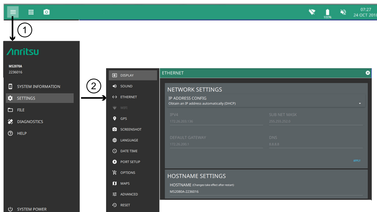
Figure 1-1. Network Settings
