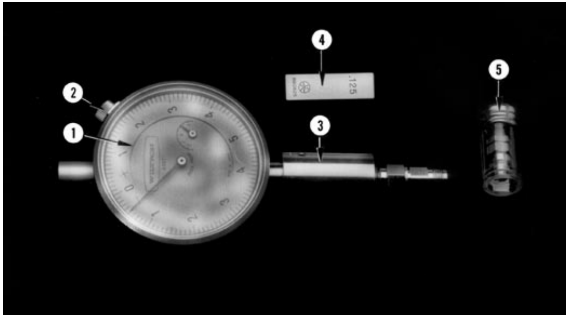
Figure 4. Model 01-164 Gauging Set
