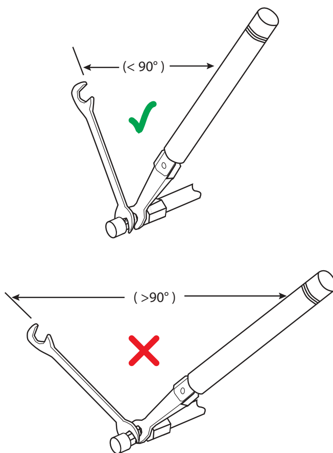
Figure 7-11. Using Wrenches at Proper Angle
