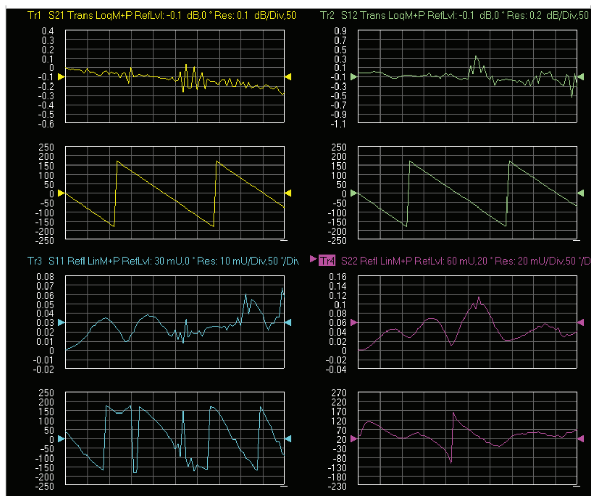
Figure 4-44. MS4640A/B Series VNA, Typical Matched Thru Data in Low Band
