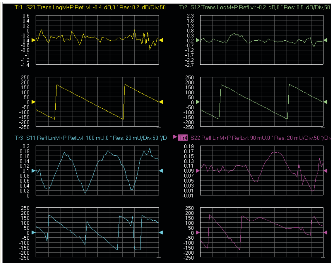
Figure 2-36. MS4640A/B Series VNA Auto Scale Example Trace Display
