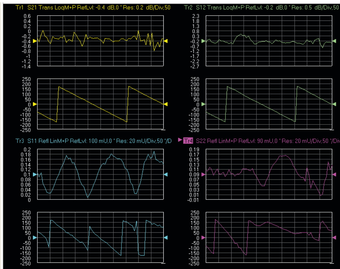
Figure 4-38. MS4640A/B Series VNA Auto Scale Example Trace Display
