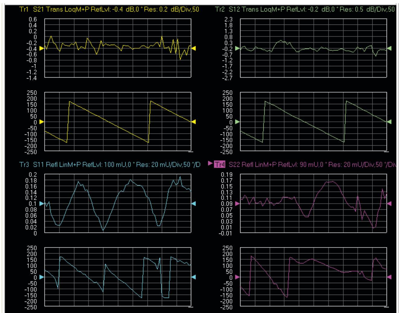
Figure 3-41. MS4640A/B Series VNA Auto Scale Example Trace Display
