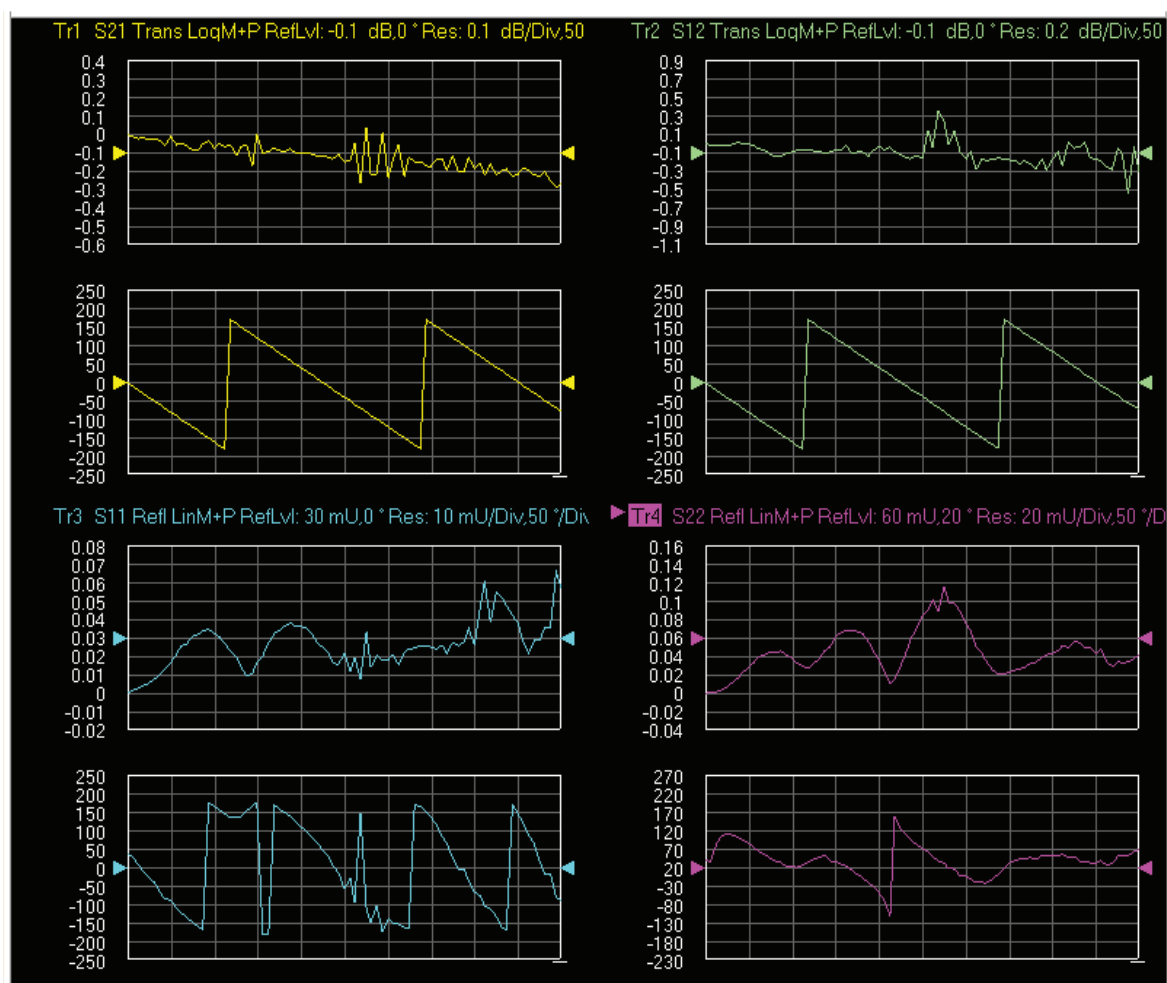
Figure 2-42. MS4640A/B Series VNA, Typical Matched Thru Data in Low Band
