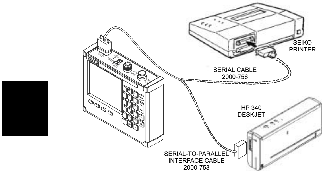
Figure 2-9. Printer Setup
