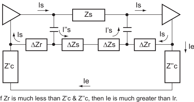
Figure 2-4. Comparison Between Common and Differential Current Flow
