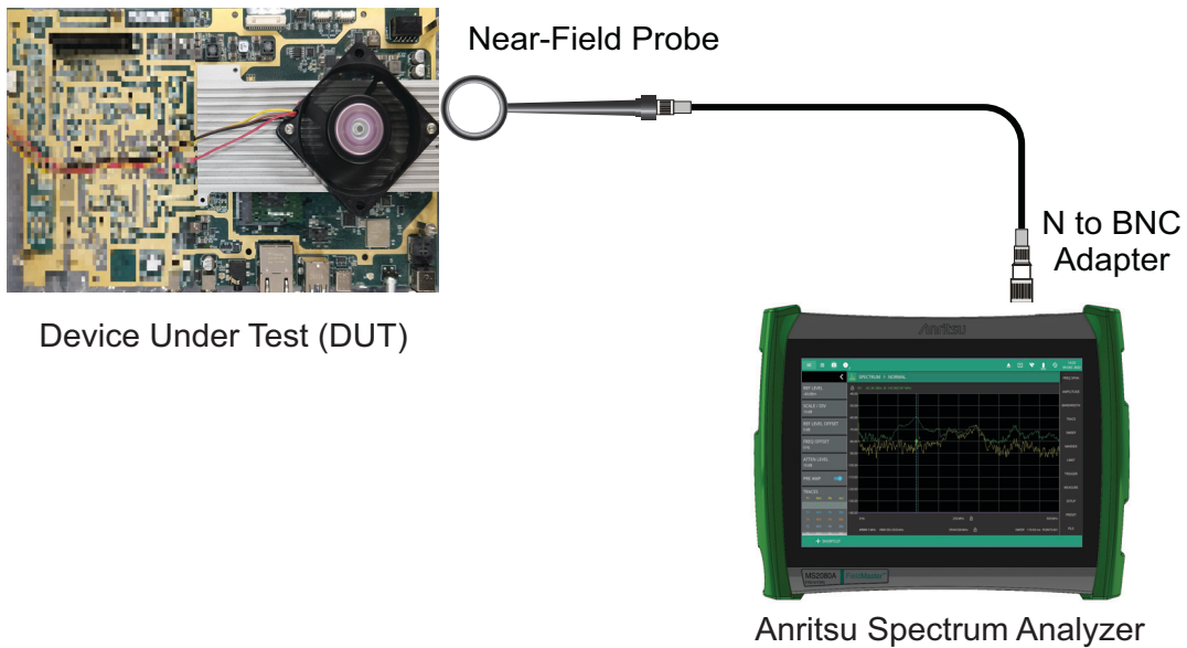
Figure 1-2. Typical Setup
