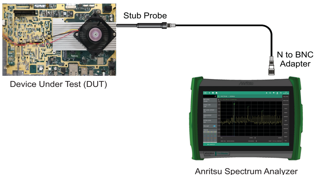
Figure 2-2. Signal Sourcing
