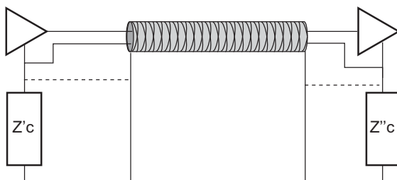
Figure 2-7. Ineffective Common Mode Techniques for Differential Mode Situations
