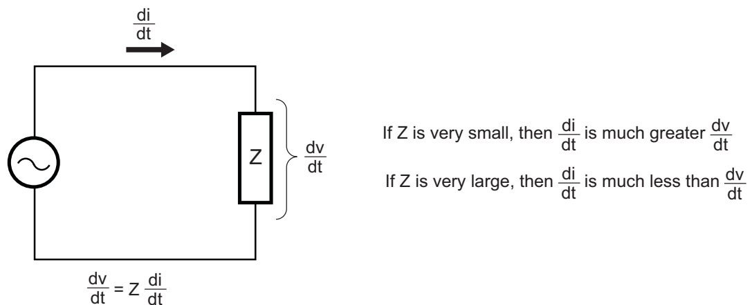
Figure 2-3. Magnetic Field or Electric Field
