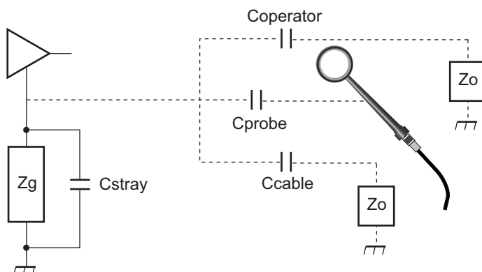
Figure 2-8. Probe and Operator May Become Part of the Circuit
