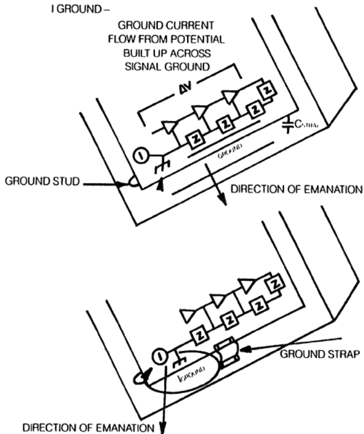
Figure 2-9. Changing the Geometry of Ground Straps
