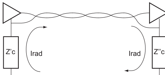
Figure 2-6. Ineffective Differential Mode Techniques for Common Mode Situations
