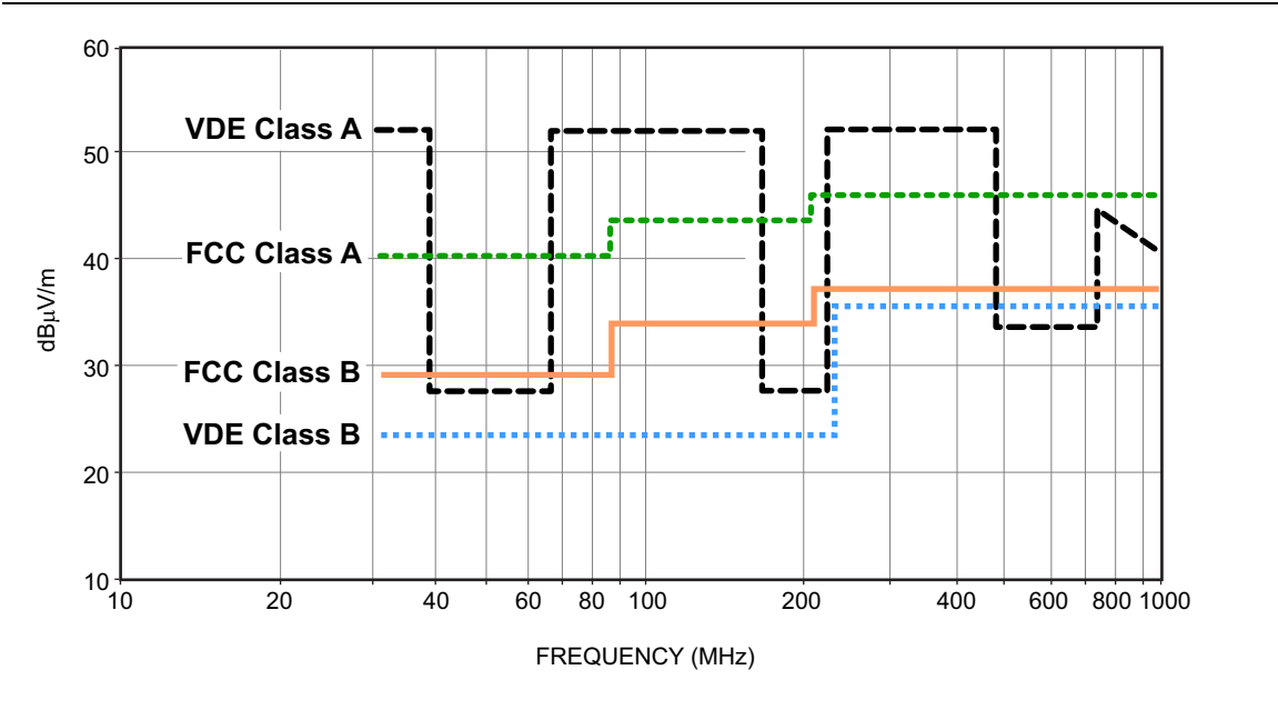
Figure 2-1. Conducted Noise Emissions Standards
