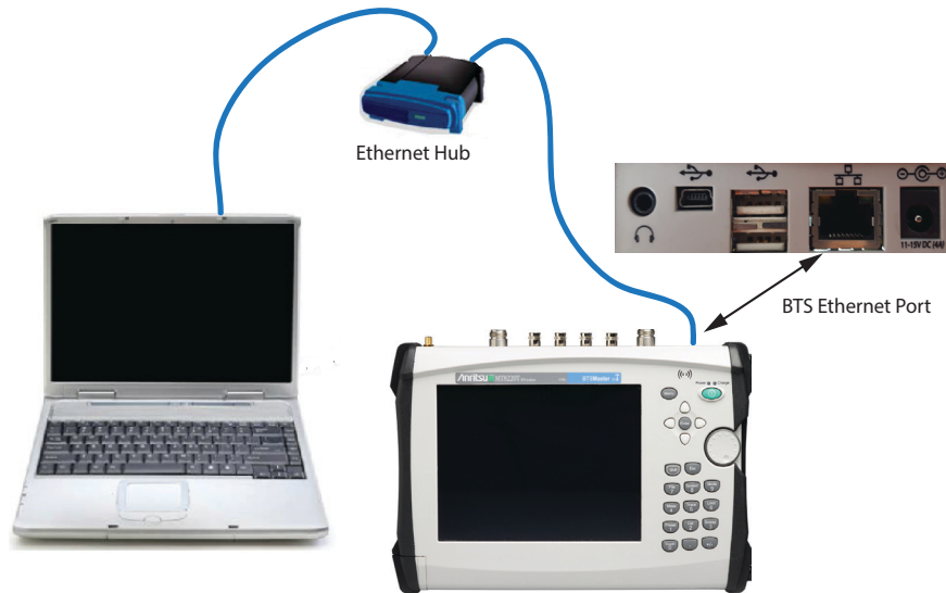
Figure 2-1. Ethernet LAN Setup
