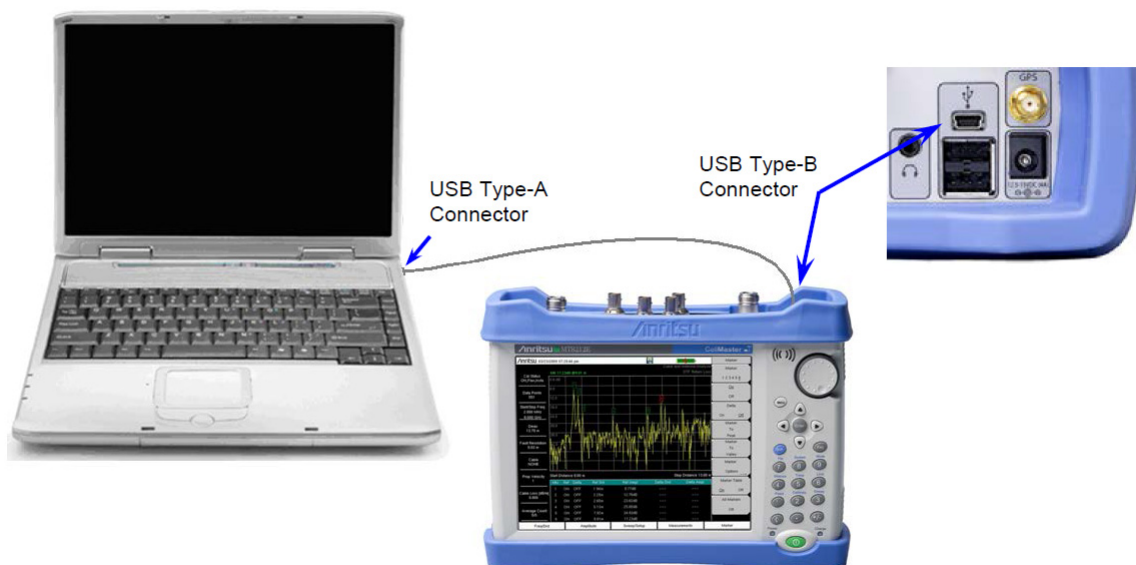
Figure 2-33. USB Connection Setup
