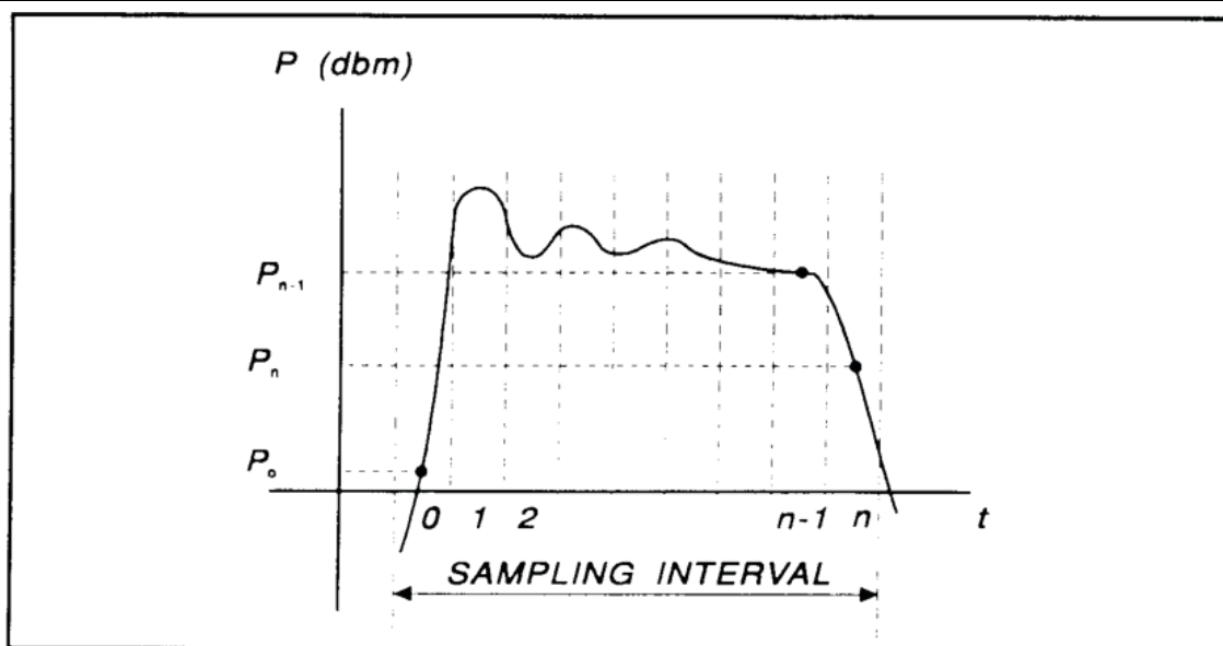
Figure 6-3. Sampling Intervals
