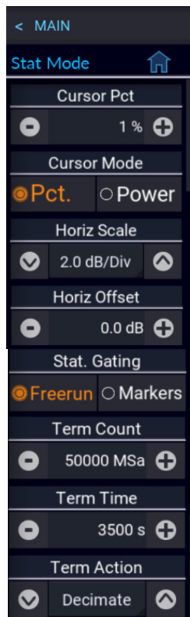
Figure 3-11. Statistical Mode Menu
