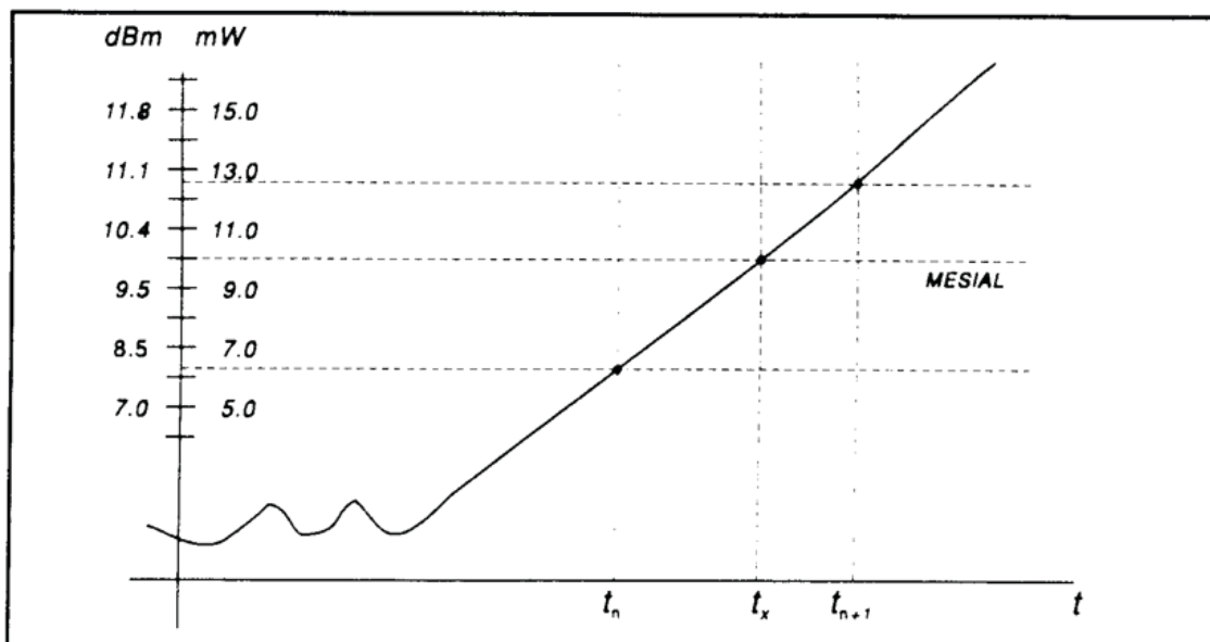
Figure 6-2. Time Interpolation
