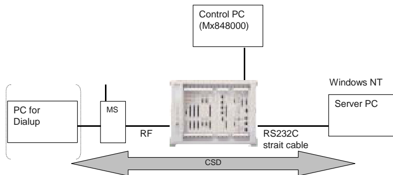
Figure : example of the GSM CSD test
