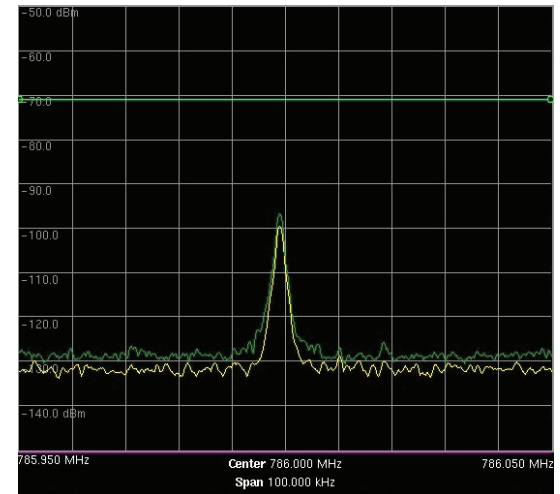
IM3 Level Seen When Away from a PIM Source
