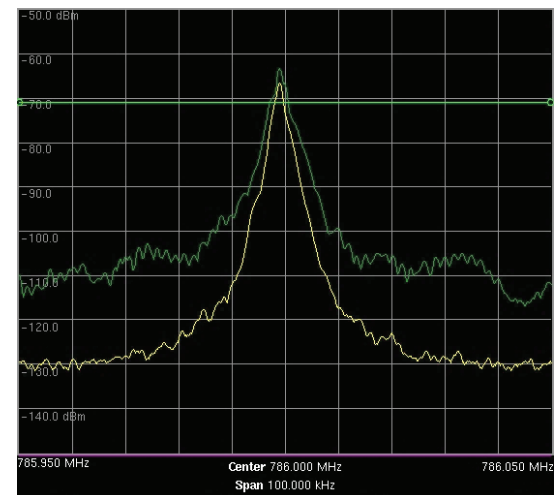
IM3 Level Seen When Near a PIM Source
