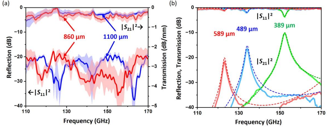
FIG. 4. (a) Measured intrinsic S parameters of (a) SIWs and (b) SIW resonators.
