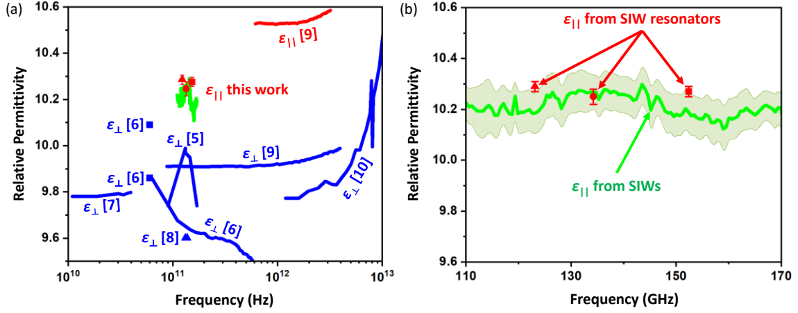
FIG. 2. (a) Relative ordinary permittivity \epsilon_{\perp} and extraordinary permittivity \epsilon_{\parallel} from 4H SiC. (b) Detailed view of data from this work. Vertical bars and shades indicate standard deviations.
