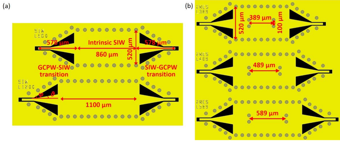
FIG. 3. Layouts of (a) SIWs and (b) SIW resonators of the same width but different lengths.
