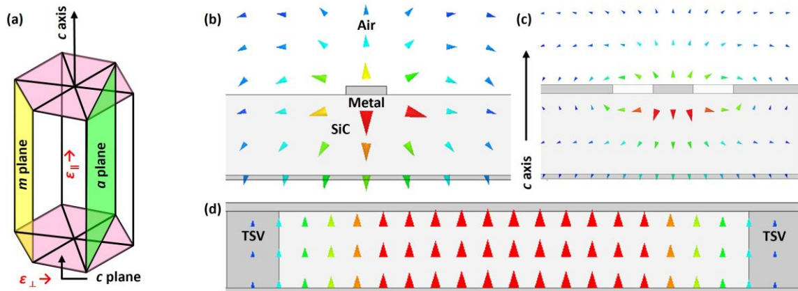
FIG. 1. (a) Crystal structure of 4H SiC. Simulated electric field distribution at 140 GHz in a (b) microstrip transmission line, (c) grounded coplanar waveguide, and (d) substrate-integrated waveguide on 100- \mu\text{m} -thick c-axis 4H SiC. Triangles point to the field direction. The warmer the color, the stronger the field.
