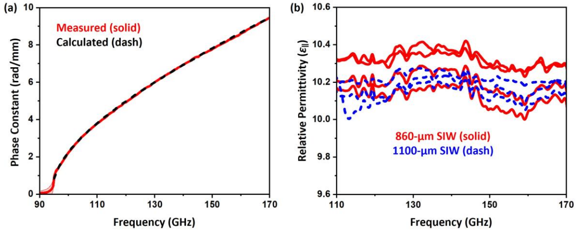
FIG. 5. (a) Measured phase constant \beta averaged over four 860- \mu\text{m} -long SIWs and three 1100- \mu\text{m} -long SIWs vs. that calculated by using \epsilon_{||} = 10.2 . (b) Relative extraordinary permittivity measured on each of the seven SIWs.
