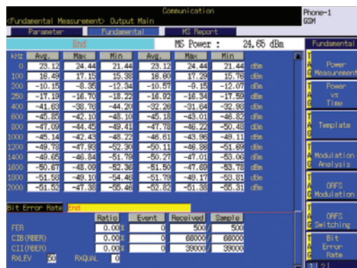
BER (GSM)
