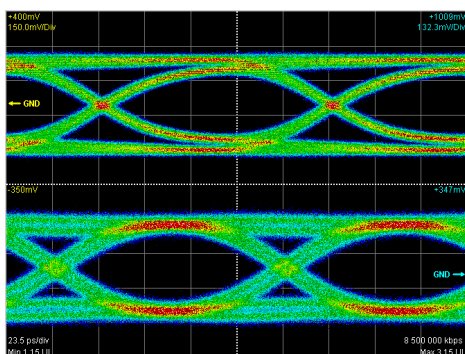
実際の波形 (EYE) (Bit Rate: 8.5Gbit/s, Pattern: PRBS 31)
