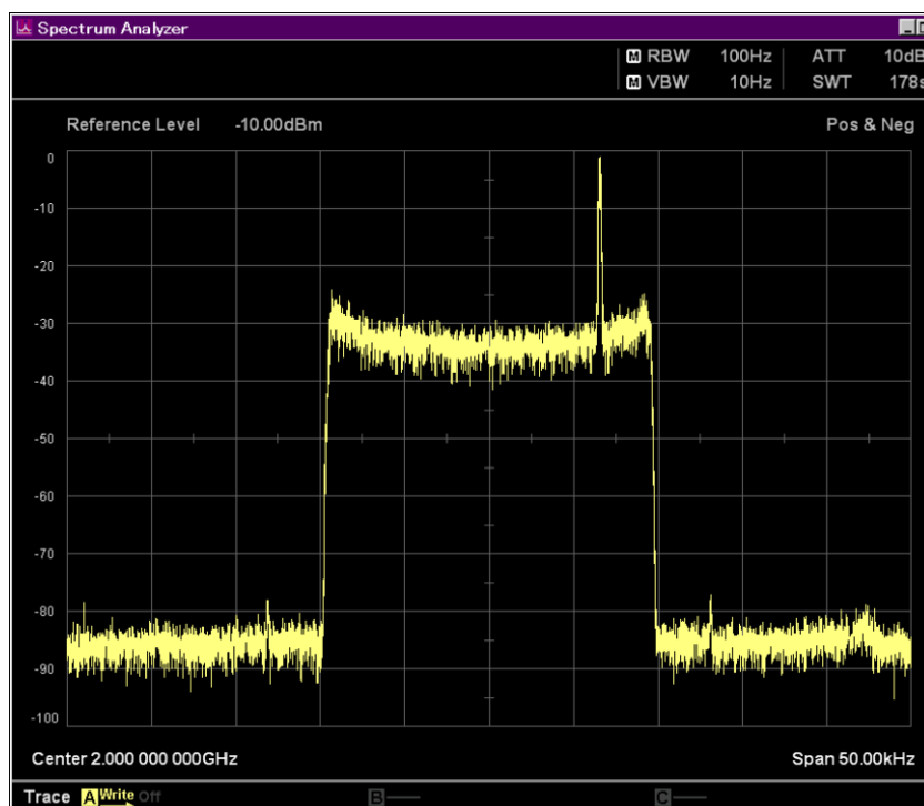
図D.1-6 Rice with Classical 6 dB
