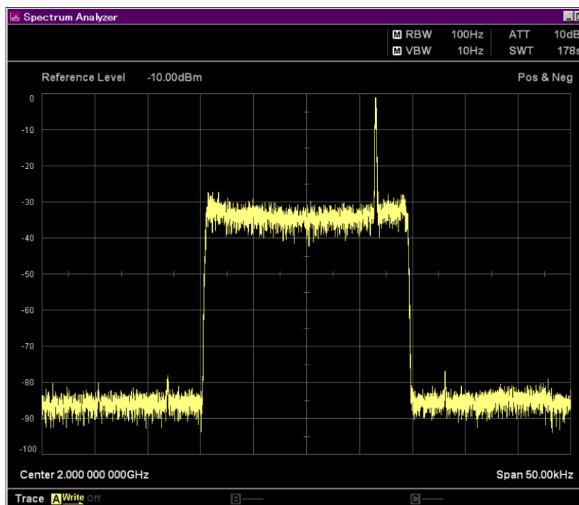
図D.1-5 Rice with Classical 3 dB
