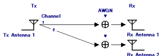
図3.1.2.2-2 1x2 SIMO
