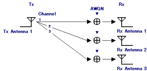
図3.1.2.2-3 1x3 SIMO
