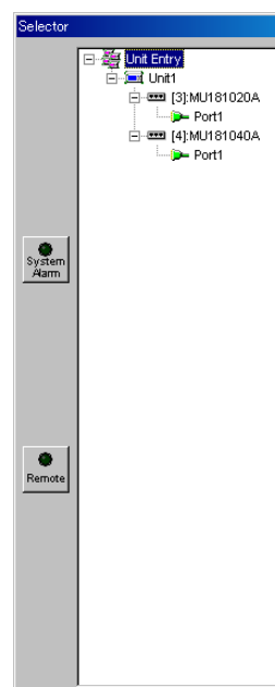
図4.3-1 Tree View
