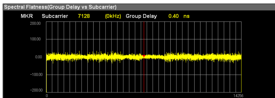
図3.6.8-2 Spectral Flatness グラフ (Group Delay vs Subcarrier)
