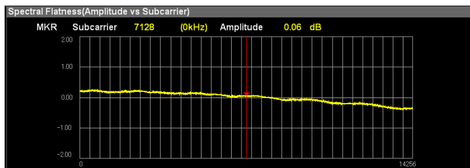
図3.6.8-1 Spectral Flatness グラフ (Amplitude vs Subcarrier)
