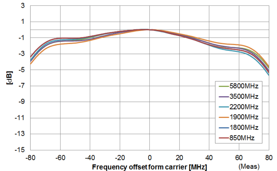
I/Q bandwidth plot using optional internal baseband generator
