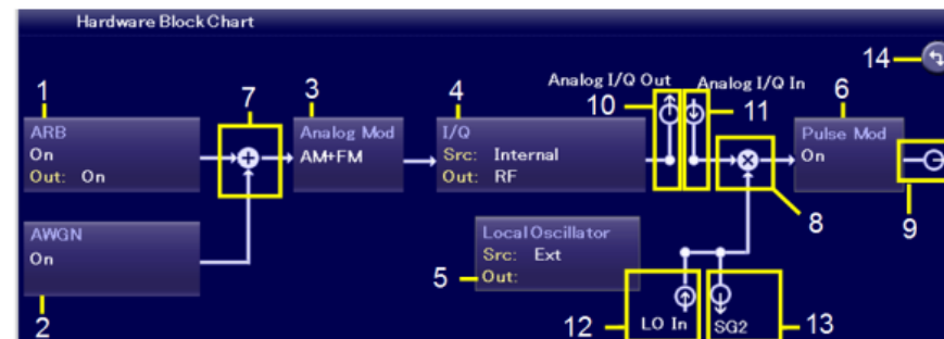
Hardware Block Chart (説明用)
