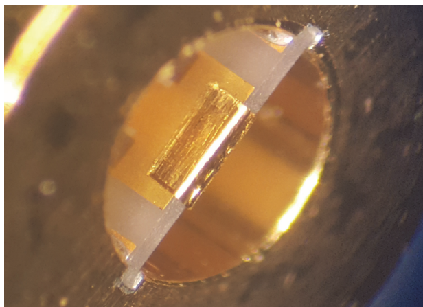
Figure 11 Shielded Suspended Substrate Stripline circuit with gold ribbon wrap-around to contact watermelon seed face
