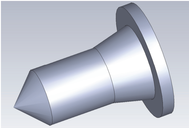
Figure 9 Capacitively compensated pin face of watermelon seed axial contact with a 12° taper angle
