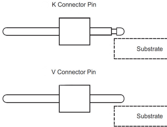
Figure 3 K and V pressure contact pins of Anritsu 3680 Universal Test Fixture (UTF)
