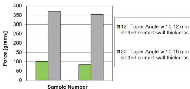
Figure 13 Influence on compression force with taper angle and slotted contact wall thickness. 50% compressed.
