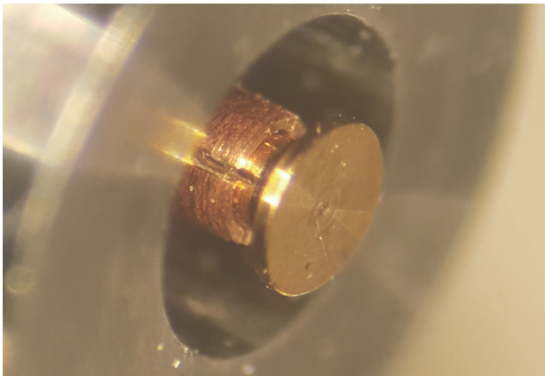
Figure 10 Capacitively compensated watermelon seed pin installed into the backside of a 1.85 mm (V) connector
