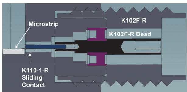
Figure 15 Single bead assembly using Anritsu K102F-R, pin and K110-1-R sliding contact
