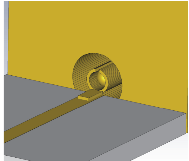
Figure 4 Non-overlapping pin using K110-1-R Sliding Contact on 10-mil thick Alumina
