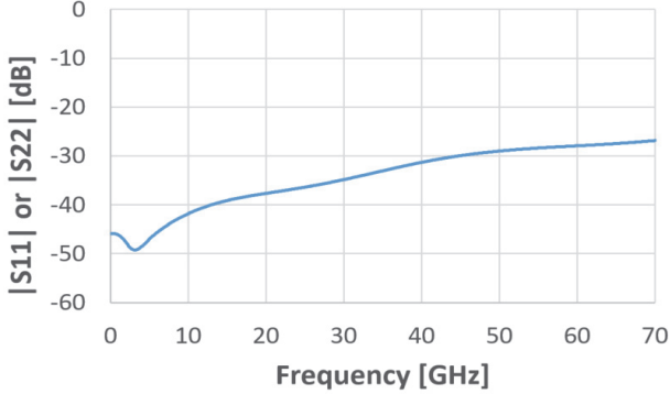
Figure 8 Typical reflection response of compensated 1.85 mm (V) Coax-to-thick Stripline transition using a tapered watermelon seed contact
