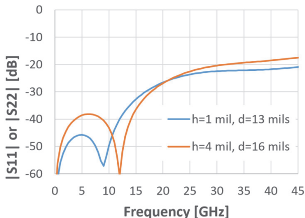
Figure 2 Parametric reflection response of gold ribbon-wrap model
