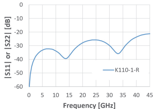
Figure 5 Typical reflection response of Sliding Contact model
