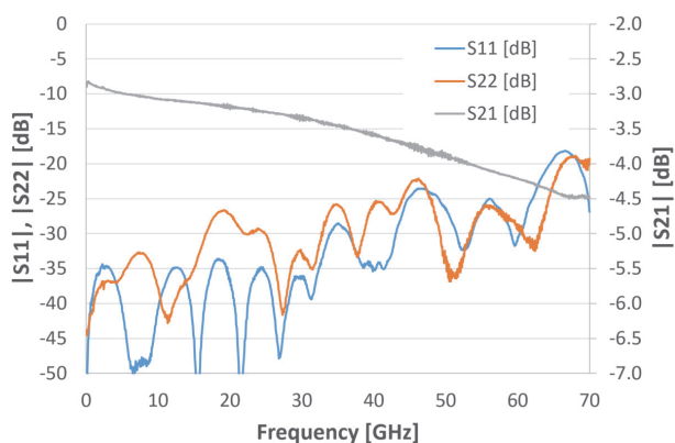
Figure 12 Response of a 1.85 mm (V) coaxial 3-dB attenuator assembly using Shielded Suspended Substrate Stripline circuit and watermelon seed axial contact
