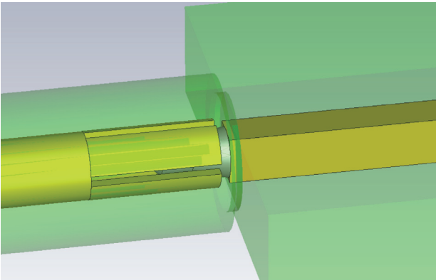
Figure 7 1.85 mm (V) Coax-to-thick Stripline transition using a 12° tapered watermelon seed contact
