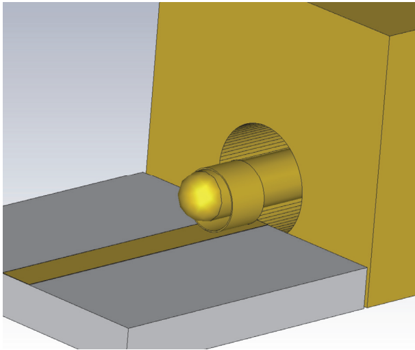
Figure 1 Backside pin overlap on 10-mil thick Alumina using gold ribbon-wrap
