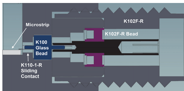
Figure 14 Dual bead assembly using Anritsu K102F-R, K100 Glass Bead and K110-1-R sliding contact
