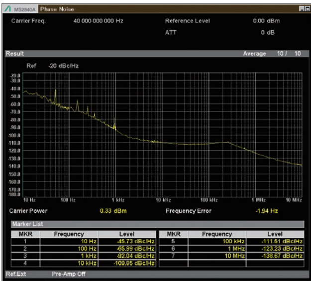
Phase Noise Measurement 40 GHz Measurement Frequency, Preamp Off
